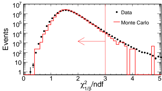
FIG. 4: Distribution of \chi_{1/\beta}^2/ndf values from the 1/\beta determinations for data and cosmic ray muon Monte Carlo events. In this figure, the Monte Carlo distribution has been normalized to the same area as the data distribution. Events with \chi_{1/\beta}^2/ndf < 3 are used in the analysis.
