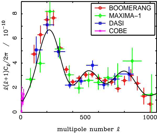
Figure 3. A compilation of the latest CMB data points from COBE, Boomerang, Maxima and DASI against spherical harmonic \ell . The line shows the predicted angular power spectrum for a \Lambda CDM model with n = 1 , \Omega_m = 1 - \Omega_\Lambda = 0.3 , \omega_b = 0.02 (BBN value), h = 0.70 , \tau = 0.0 , and the best-fit normalization to the given CMB data points \sigma_{8m} = 0.83 . Note that this normalization is lower than the traditional COBE-only normalization (see Table 1). A similar model is also the best fit to the shape of the 2dFGRS galaxy power spectrum (Fig. 1).
