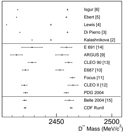
FIG. 5: D_1^0 (solid) and D_2^{*0} (open) mass comparison with theoretical expectations (triangles) and previous measurements and current world average (circles). Errors for theory predictions are not readily available.
