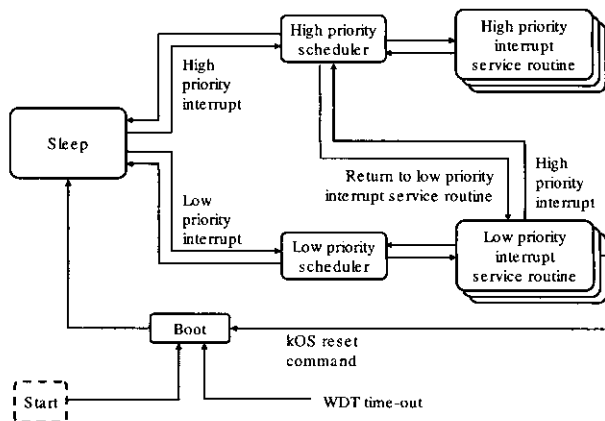
Fig. 4. Basic kOS operation, showing the sleep/wake cycle and the use of interrupt service routine for high and low-priority tasks.
