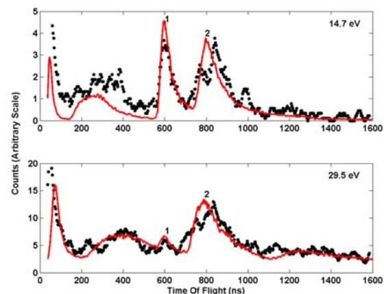
Figure 2. IMS time of flight data for two energies summed over the time interval t_1 to t_2 in Figure 1. The model calculations shown in red establish the presence of O^+ and O_2^+ over the main rings although the additional presence of OH^+ and H_2O^+ cannot be excluded.
