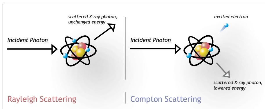
Figure 5. The principle of Rayleigh scattering (on the left) compared to Compton scattering (on the right).
