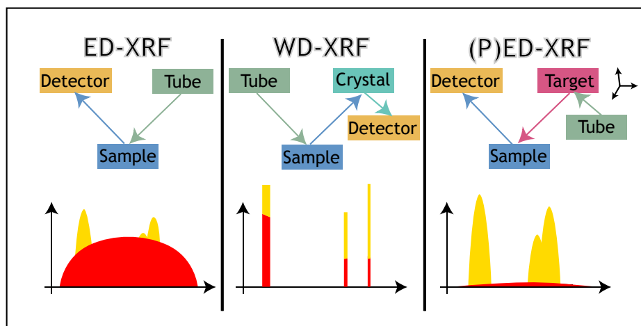
Figure 3. The principle of background noise reduction by (P)ED-XRF, compared to (standard) ED-XRF and WD-XRF (after Schramm n.d. b), fig. 7, p.10).
