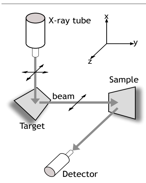
Figure 2. The principle of polarisation (P)ED-XRF, showing the orientation of target and sample in relation to the beam.
