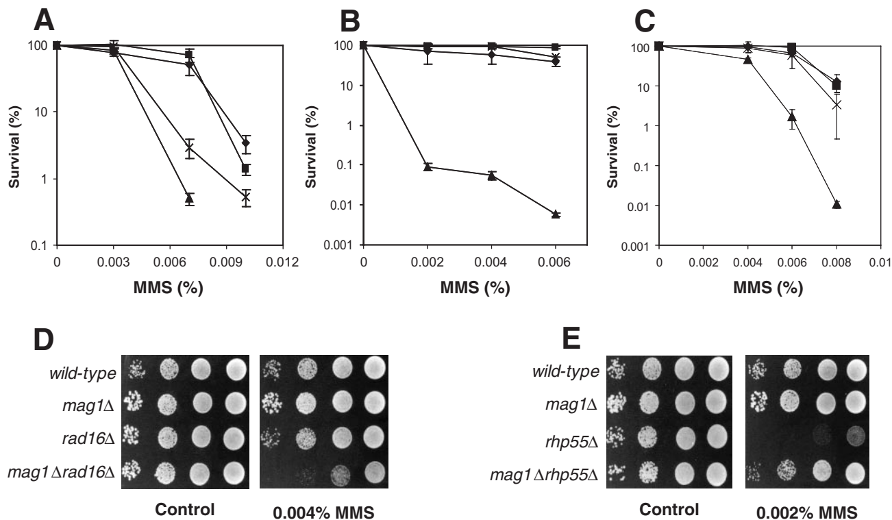
Figure 2. Genetic interactions between mag1 , nth1 , apn2 , rad2 , rad16 and rhp55 analysed for MMS sensitivity. (A) S.pombe wild type (diamonds), mag1 (squares), nth1 (triangles) and mag1 nth1 (crosses) mutant cells were plated onto solid media containing increasing doses of MMS and assessed for cell survival by colony formation. (B) S.pombe wild type (diamonds), mag1 (squares), apn2 (triangles) and mag1 apn2 (crosses) mutant cells were plated onto solid media containing increasing doses of MMS and assessed for cell survival by colony formation. (C) S.pombe wild type (diamonds), mag1 (squares), rad2 (triangles) and mag1 rad2 (crosses) mutant cells were plated onto solid media containing increasing doses of MMS and assessed for cell survival by colony formation. (D) An aliquot 10 \mu l or serially diluted ( 10^6 – 10^3 cells \text{ml}^{-1} ) mid-log phase cultures of wild type, mag1 , rad16 , mag1 rad16 and (E) wild type, mag1 , rhp55 and mag1 rhp55 were spotted onto YES plates containing no MMS (control) or MMS doses as indicated.
