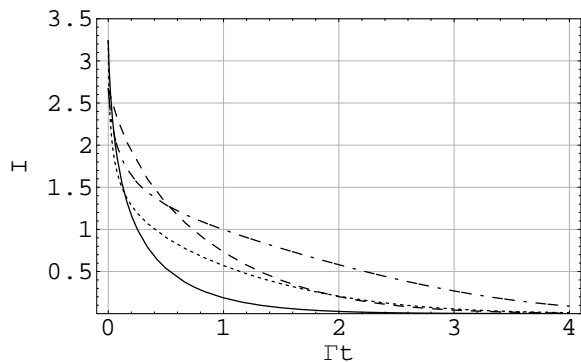
FIG. 7: Time evolution of the mutual information of two-mode squeezed thermal states in an environment with \mu_1 = \mu_2 = 1/3 . The solid line refers to a pure state with r = 1 in a non squeezed environment; the dotted line refers to the same state in an environment with r_1 = r_2 = 1 ; the dashed line refers to a squeezed thermal state with \mu = 1/16 , r = 1 in a non squeezed environment; the dot-dashed line refers to the same state in a squeezed environment with r_1 = r_2 = 1 . The squeezing angle \varphi_2 has always been set to 0. All the plotted quantities are dimensionless.
