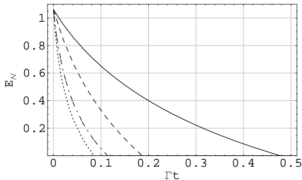
FIG. 2: Time evolution of logarithmic negativity of a symmetric Gaussian state with a = 1.5 , b = 1.5 , c_1 = 1.2 , c_2 = -1.4 in several non correlated environments. The solid line refers to the case \mu_1 = \mu_2 = 1/2 , r_1 = r_2 = 0 ; the dashed line refers to the case \mu_1 = \mu_2 = 1/4 , r_1 = r_2 = 0 ; the dot-dashed line refers to the case \mu_1 = \mu_2 = 1/2 , r_1 = r_2 = 1 ; the dotted line refers to the case \mu_1 = \mu_2 = 1/2 , r_1 = 0 , r_2 = 1.5 . In all cases the squeezing angle \varphi_2 = 0 . All the plotted quantities are dimensionless.
