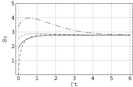
FIG. 6: Time evolution of the Von Neumann entropy of several Gaussian states in a thermal environment with \mu_1 = \mu_2 = 1/3 . The solid line refers to a state with a = 1 , b = c_1 = -c_2 = 1 ; the dashed line refers to a two-mode squeezed vacuum state with r = 1 ; the dot-dashed line refers to a squeezed thermal state with \mu = 1/16 , r = 1 ; the dotted line refers to a non entangled state with a = b = 2 , c_1 = -c_2 = 1.5 . The squeezing angle \varphi_2 has always been set to 0. All the plotted quantities are dimensionless.
