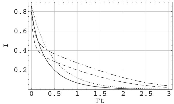
FIG. 8: Time evolution of the mutual information of Gaussian states in an environment with \mu_1 = \mu_2 = 1/3 . The solid line refers to state with a = 2 , b = c_1 = -c_2 = 1 in a non squeezed environment; the dotted line refers to the same state in an environment with r_1 = r_2 = 1 ; the dashed line refers to a non entangled state with a = b = 2 , c_1 = -c_2 = 1.5 in a non squeezed environment; the dot-dashed line refers to the same state in a squeezed environment with r_1 = r_2 = 1 . The squeezing angle \varphi_2 has always been set to 0. All the plotted quantities are dimensionless.
