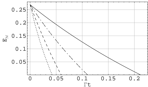
FIG. 1: Time evolution of logarithmic negativity of a non symmetric Gaussian state with a = 2, b = 1, c_1 = 1, c_2 = -1 in several non correlated environments. The solid line refers to the case \mu_1 = \mu_2 = 1/2, r_1 = r_2 = 0 ; the dashed line refers to the case \mu_1 = 1/2, \mu_2 = 1/6, r_1 = r_2 = 0 ; the dot-dashed line refers to the case \mu_1 = 1/6, \mu_2 = 1/2, r_1 = r_2 = 0 ; the dotted line refers to the case \mu_1 = \mu_2 = 1/2, r_1 = r_2 = 1 . In all cases the squeezing angle \varphi_2 = 0 . All the plotted quantities are dimensionless.
