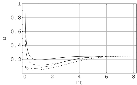
FIG. 5: Time evolution of the purity of two-mode squeezed thermal states. The solid line refers to a two-mode squeezed vacuum state with r = 1 in an environment with \mu_1 = \mu_2 = 1/2 , r_1 = r_2 = 0 ; the dashed line shows the behavior of the same state for \mu_1 = \mu_2 = 1/2 , r_1 = r_2 = 1 . The dot-dashed line refers to a mixed state with \mu = 1/9 , r = 1 in an environment with \mu_1 = \mu_2 = 1/2 , r_1 = r_2 = 0 ; the dotted line refers to the same state for \mu_1 = \mu_2 = 1/2 , r_1 = r_2 = 1 . The squeezing angle \varphi_2 has always been set to 0. All the plotted quantities are dimensionless.
