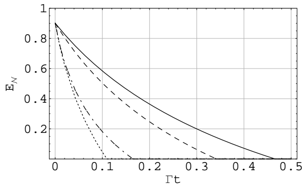
FIG. 4: Time evolution of logarithmic negativity of a two-mode squeezed thermal state with initial purity \mu = 1/9 , r = 1 in several non correlated environments. The solid line refers to the case \mu_1 = \mu_2 = 1/2 , r_1 = r_2 = 0 , \varphi_2 = 0 ; the dashed line refers to the case \mu_1 = 4 , \mu_2 = 1 , r_1 = r_2 = 0 , \varphi_2 = 0 ; the dot-dashed line refers to the case \mu_1 = \mu_2 = 1/2 , r_1 = r_2 = 1 , \varphi_2 = 0 ; the dotted line refers to the case \mu_1 = \mu_2 = 1/2 , r_1 = r_2 = 1 , \varphi_2 = \pi/4 . All the plotted quantities are dimensionless.
