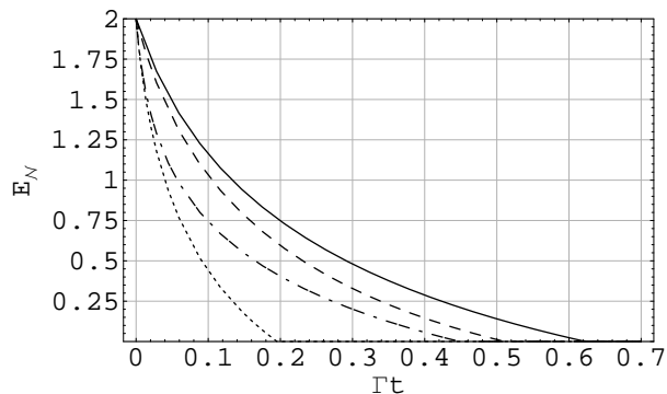
FIG. 3: Time evolution of logarithmic negativity of a two-mode squeezed state with r = 1 in several non correlated environments. The solid line refers to the case \mu_1 = \mu_2 = 1/2 , r_1 = r_2 = 0 , \varphi_2 = 0 ; the dashed line refers to the case \mu_1 = 4 , \mu_2 = 1 , r_1 = r_2 = 0 , \varphi_2 = 0 ; the dot-dashed line refers to the case \mu_1 = \mu_2 = 1/2 , r_1 = r_2 = 1 , \varphi_2 = 0 ; the dotted line refers to the case \mu_1 = \mu_2 = 1/2 , r_1 = r_2 = 1 , \varphi_2 = \pi/4 . All the plotted quantities are dimensionless.
