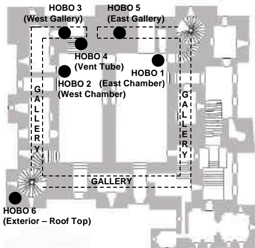
Figure 4 First floor plan with datalogger locations indicated
