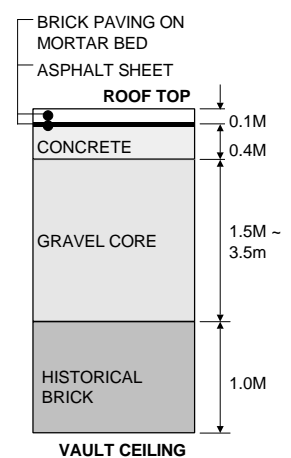
Figure 2 Cross section of the brick vault
