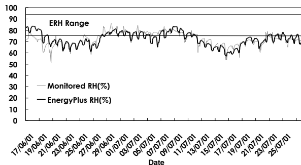
Figure 8 Monitored vs. EnergyPlus RH prediction for summer 2001
