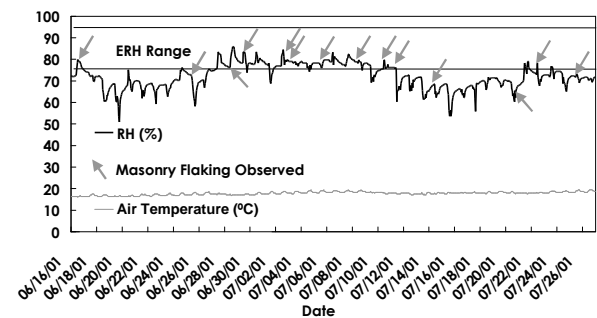
Figure 5 West chamber air temperature, RH and observed incidences of flaking activity
