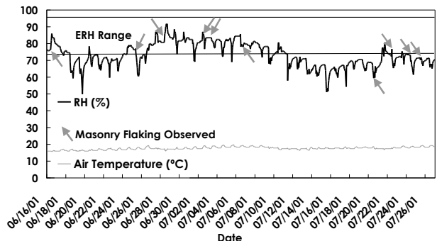
Figure 6 East Chamber air temperature, RH and observed incidences of flaking activity
