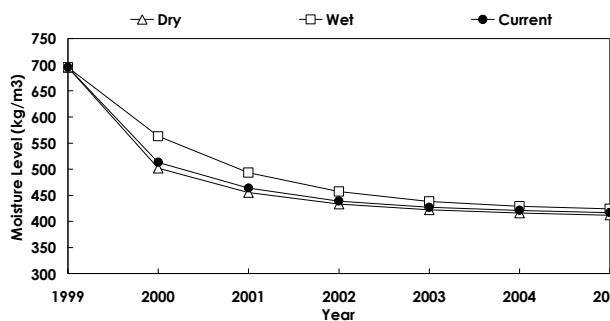
Figure 15 Vault interstitial moisture level over a period of six years of drying period
