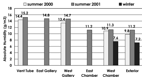
Figure 7 Comparison of average absolute humidity levels of all monitored locations
