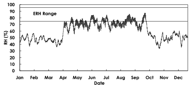
Figure 11 Annual variation in predicted RH
