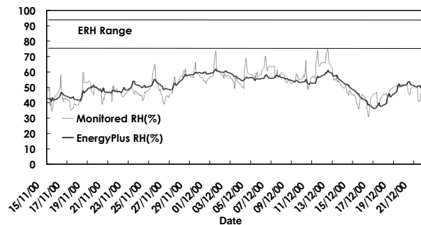
Figure 9 Monitored vs. EnergyPlus RH prediction for winter 2000
