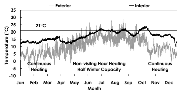
Figure 14 977 predicted annual hours above 21^\circ\text{C} under full winter and partial summer heating
