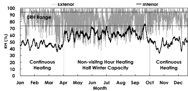
Figure 13 38 predicted annual ERH hours under full winter and partial summer heating
