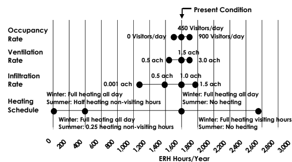
Figure 12 ERH sensitivity under varying internal condition
