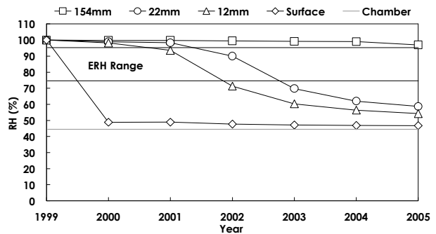
Figure 16 Interstitial RH at four vault depths
