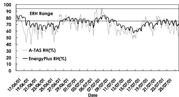
Figure 10 EnergyPlus vs. A-TAS RH prediction for summer 2001
