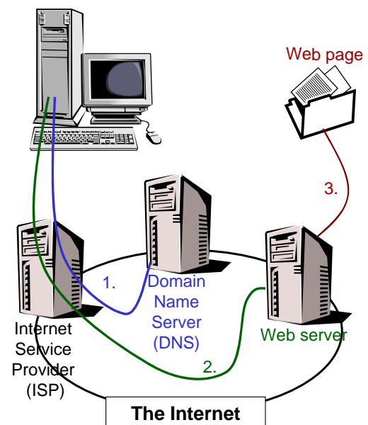
Figure 2: Suggested Design Model for Web Browsing
