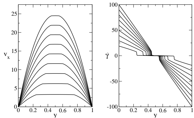
FIG. 2: Left) Velocity profiles in one-dimensional planar shear banded Poiseuille flow for a = 0.3, \eta = 0.05, l = 0.0025 . Increased throughputs correspond to increased applied pressure gradients G = 2.0, 3.0, 4.0, 5.0, 6.0, 7.0, 8.0, 9.0, 10.0 . Right) Corresponding shear rate profiles, which follow as the spatial derivative of the velocity profiles.
