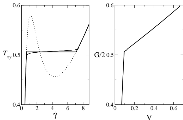
FIG. 1: Left) Dotted line: homogeneous constitutive curve for a = 0.3 , \eta = 0.05 . Thick solid line: composite flow curve for one-dimensional planar shear banded Couette flow (data already published in Ref. [50]). Selected stress T_{\text{sel}} = 0.506 . Thin solid line: parametric plot of local shear stress T_{xy}(y) = \Sigma_{xy}(y) + \eta\dot{\gamma}(y) = G(\frac{1}{2} - y) against local shear rate \dot{\gamma}(y) for one-dimensional planar shear banded Poiseuille flow with l = 0.00125 , G = 2.0 .
