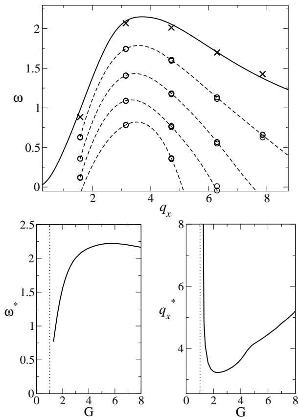
FIG. 3: Top) Dispersion relation of growth rate \omega versus wavevector q_x during the initial stage of 2D instability, starting with a 1D shear banded planar Poiseuille basic state. In each case a = 0.3 , \eta = 0.05 , G = 4.0 . Circles: extracted from early time dynamics of the full nonlinear code. Groups of data upward correspond to l = 0.02, 0.015, 0.01, 0.005 . Within each group, data are shown for (Dt, N_x, N_y) = (0.000025, 200, 400), (0.0000125, 200, 400), (0.000025, 400, 800) . These are mostly indistinguishable, demonstrating convergence with respect to grid and timestep. Dashed lines: cubic splines through the data for (Dt, N_x, N_y) = (0.000025, 200, 400) , as a guide to the eye. L_x = 4.0 in each case. Solid line: results of analytical calculation in the true limit l \rightarrow 0 . Crosses: extrapolation of the l \neq 0 results to l = 0 using the scaling \omega(q_x, l) = \omega(q_x, l = 0) - a(q_x)l . Bottom) Growth rate (left) and wavevector (right) at the peak of dispersion relations as a function of the pressure drop G , calculated analytically in the limit l \rightarrow 0 .
