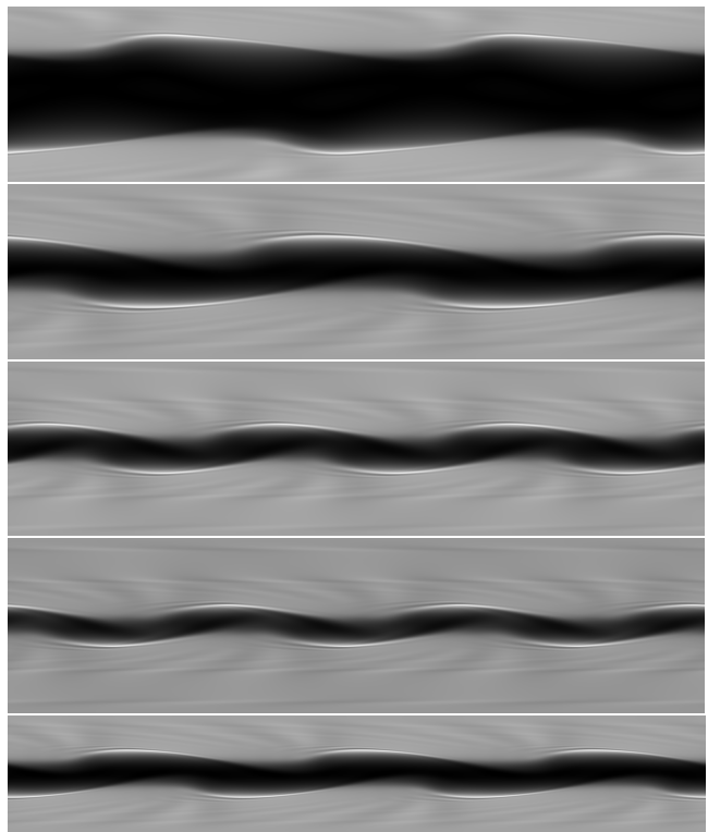
FIG. 4: Greyscale snapshots of the order parameter \Sigma_{xx}(x, y) at a representative time t = 60.0 on the ultimate nonlinear attractor for a = 0.3 , \eta = 0.05 , l = 0.005 for L_x = 4.0 and G = 2.0, 4.0, 6.0, 8.0 (top four subfigures downwards) with Dt = 0.000025 , N_x = 200 , N_y = 400 . Bottom subfigure is for G = 4.0 with a longer cell L_x = 6.0 (so N_x = 300 ).
