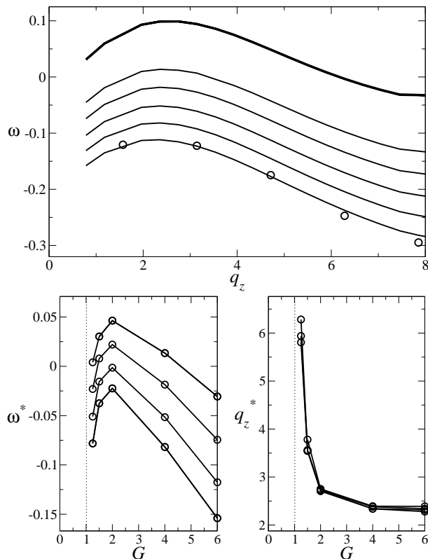
FIG. 6: Top) Dispersion relation of growth rate \omega versus wavevector q_z during the initial stage of 2D instability, starting with a 1D shear banded planar Poiseuille basic state. In each case a = 0.3 , \eta = 0.05 , G = 4.0 . Thin solid lines: calculated by linear stability analysis using the method of Ref. [52], with lines upward corresponding to l = 0.0035, 0.003, 0.0025, 0.002, 0.0015 . Thick solid lines: extrapolation of the l \neq 0 results shown by each of the thin solid lines to l = 0 using the scaling \omega(q_x, l) = \omega(q_x, l = 0) - a(q_x)l . Indistinguishability of the thick lines demonstrates the validity of this scaling. Circles: extracted from early time dynamics of the full nonlinear code for l = 0.0035 .
