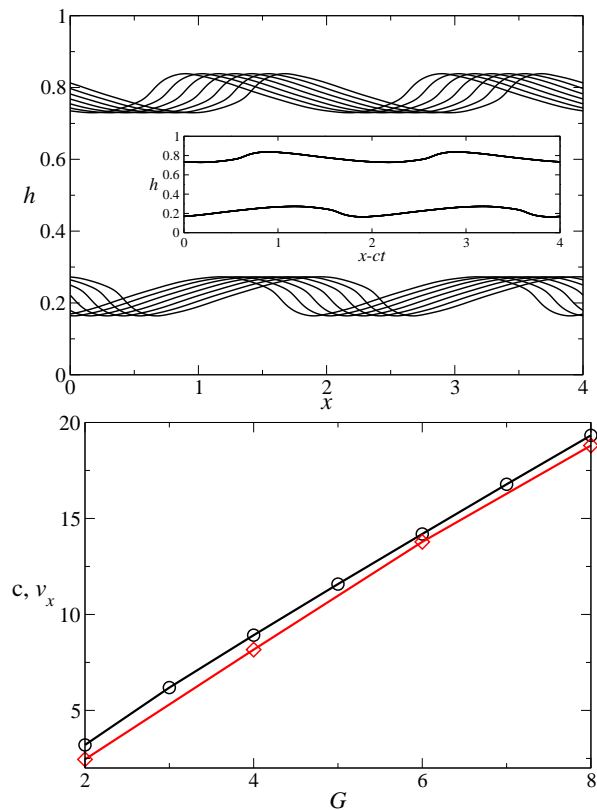
FIG. 5: Top) Snapshot of interface height h(x) for a = 0.3 , \eta = 0.05 , l = 0.005 , L_x = 4.0 and G = 2.0 at six times equally spaced by \Delta t = 0.05265 . Dt = 0.000025 , N_x = 200 , N_y = 400 . Inset: the same data plotted versus transformed coordinate x - ct revealing simple convective motion with a constant wavespeed c .
