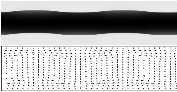
FIG. 7: Order parameter \Sigma_{xx}(y, z) greyscale (top) and velocity map showing secondary flow in y - z plane (bottom): snapshot at time t = 1895 in steady state for a = 0.3 , \eta = 0.05 , l = 0.0015 for L_x = 4.0 and G = 2.0 with Dt = 0.05 , N_z = 1000 , N_y = 1066 .
