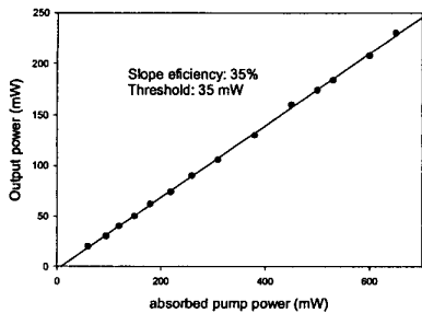
CWC5 Fig. 2. Laser power characteristics. These did not change noticeably with pump polarization angle.
