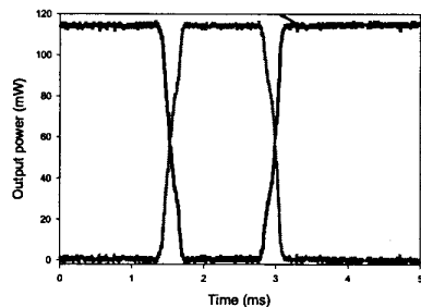
CWC5 Fig. 3. Polarization switching of PM EDFL when pump polarization is not aligned on the fiber's principal axes. The two curves show the power in the main axis of the fibre as a function of time.
