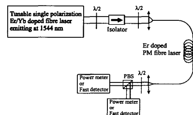
CWC5 Fig. 1. Experimental set-up.
