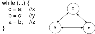
Figure 1. A Slice-based Cluster
