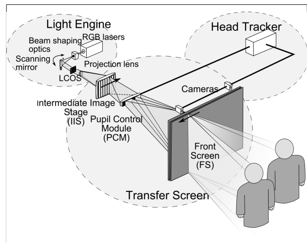
Figure 1. A simplified schematic diagram showing the subsystems comprising the HELIUM3D display.
