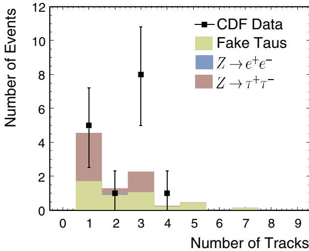
FIG. 10 (color online). Track multiplicity distribution for the non-back-to-back events with the \cancel{E}_{T,h} > 0 requirement, but without the N_{\text{cone}}^{\text{trks}} < 4 , |Q| = 1 and opposite-sign requirements.
