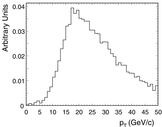
FIG. 2. The p_T of directly produced Higgs bosons with mass m_A = 100 \text{ GeV}/c^2 after a \sin\Delta\phi > 0.3 cut has been imposed.
