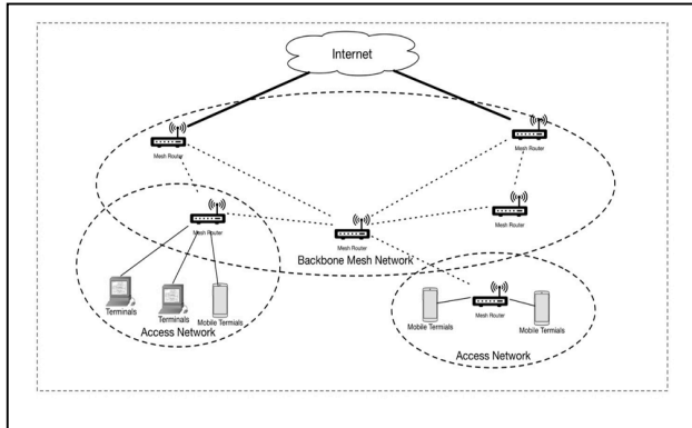
Fig. 2 Infrastructure/Backbone WMN structure
