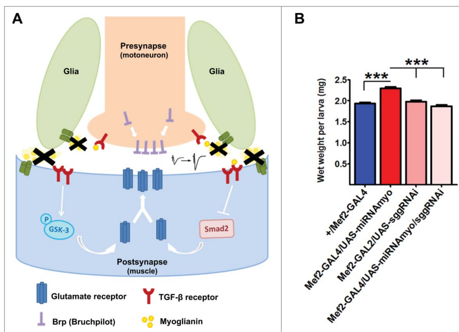
Figure 1. Reduced Myoglianin levels promote membrane targeting of the presynaptic active zone assembly regulator (Brp) and postsynaptic glutamate receptors (type A) via inhibition of Smad2/ Smox and stimulation of GSK-3/shaggy signaling, resulting in enhanced electrophysiological response.
