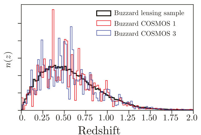
Figure 5. Redshift distributions of the full simulated lensing sample from the BUZZARD catalogue (grey) and two examples of samples from COSMOS-sized footprints in the BUZZARD catalogues that have been resampled and weighted to match the full distribution (blue and orange).
