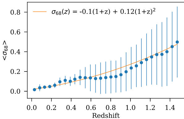
Figure 2. The average width of the posterior distributions of BPZ photometric redshifts for data selected in bins of mean BPZ redshift. The posterior width is defined as the 68 per cent spread of the PDF p^{PZ}(z) about its median. The error bars correspond to the standard deviation of the individual source’s \sigma_{68} around the average.
