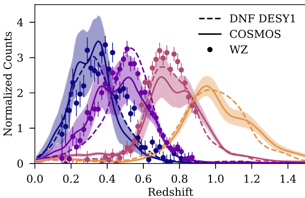
Figure C1. Top panel: as Fig. 2 showing the average width of the posterior distributions of DNF photometric redshifts. Bottom panel: the n^i(z) for galaxies with bin assignments and estimated using DNF photo- z 's rather than BPZ. The error bars correspond to the standard deviation of the individual source's \sigma_{68} around the average. The bottom panel is otherwise equivalent to Fig. 4.
