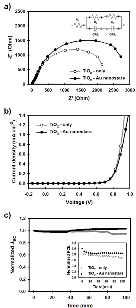
Figure 3. (a) Nyquist plots of EIS measurements (measured under illumination at 0.8 V bias), (b) dark J - V curves, and (c) Normalized J_{sc} values and PCEs (inset) of the devices as a function of time exposed to continuous light illumination (100 mW cm -2 , Xe lamp).
