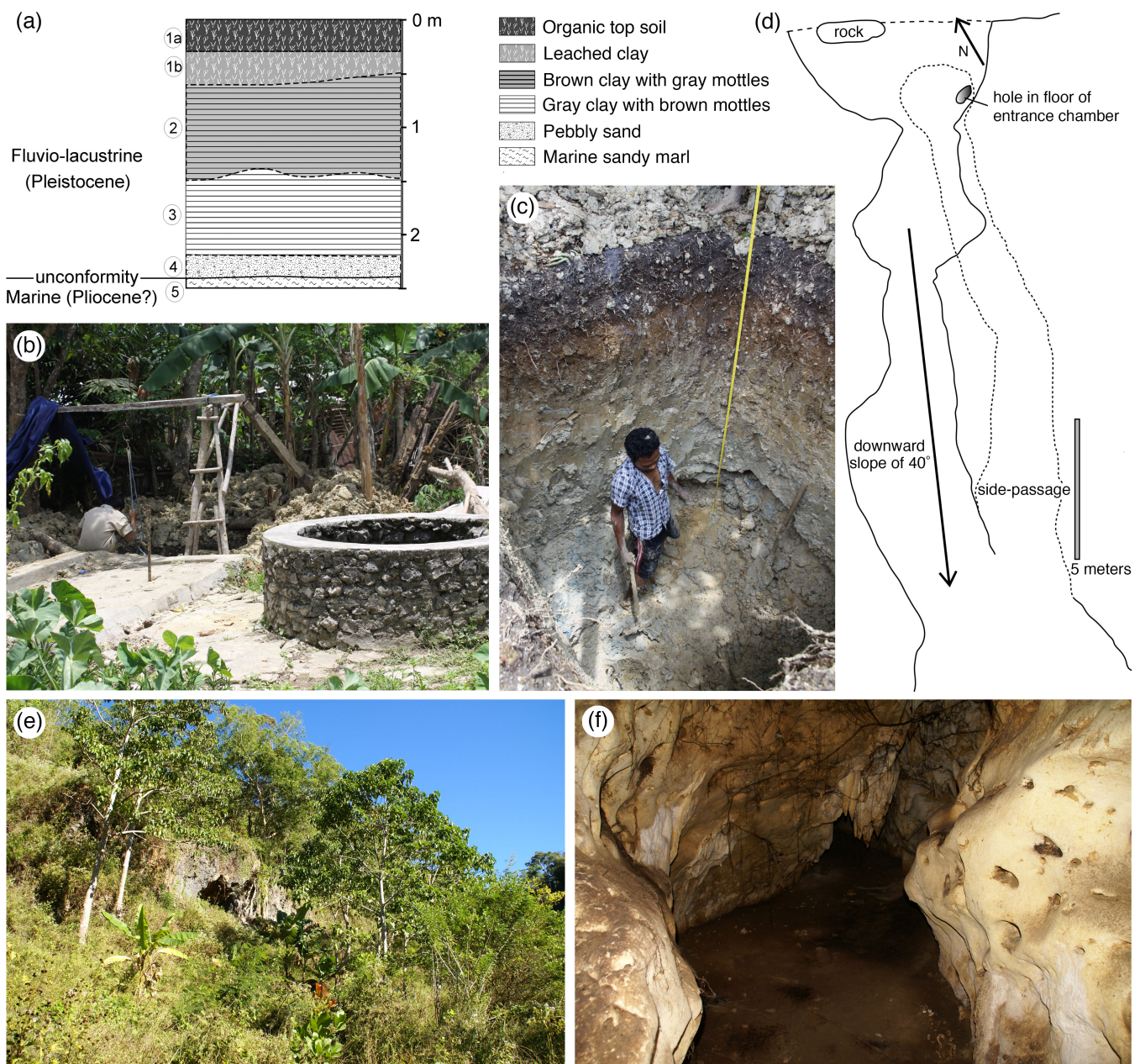
Fig. S1. Quaternary vertebrate fossil localities on Sumba. (a) Stratigraphic profile of the west bank of the excavation at Lewapaku. Fossil vertebrate remains were concentrated in Layer 4. (b) View to the north at the Lewapaku excavation, with water well in foreground. (c) View towards northeast corner of Lewapaku excavation. (d) Plan view of Liang Lawuala. (e) Entrance to Liang Lawuala, looking southwest. (f) View to the northeast along the side-passage at Liang Lawuala, where fossil vertebrate remains were concentrated.
