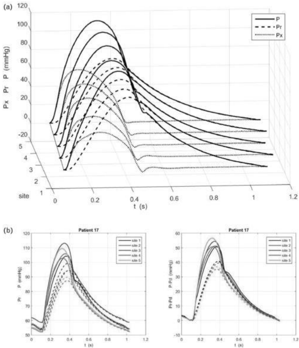
FIGURE 2. (a) The ensemble average of the measured pressure waveform at the five aortic sites for one patient (black), together with the reservoir (dashed) and excess (dotted) pressure waveforms. Time is relative to the R-wave of the simultaneously measured ECG. The dotted black line indicates the time of the diastolic point at the different sites, and the slope of this line is the pulse wave speed. For ease of comparison of the waveforms, P-P_d and P_r-P_d are plotted. (b) Example data from the same individual participant showing pressure waveforms at the five sites relative to atmospheric pressure (left panel); note the changes in P_d between sites. The right hand panel shows the same data plotted relative to P_d [i.e. P(t)-P_d and P_r(t)-P_d ]. The waveforms are aligned at the start of systole to allow comparison.
