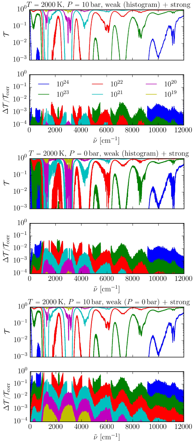
Fig. 12. Transmissions computed using the Doppler model ( upper panel ) and histogram continuum models ( R = 1\,000\,000 , middle and lower panels ) with relative errors for the column amounts 10^{19} , 10^{20} , 10^{21} , 10^{22} , 10^{23} , and 10^{24} molecule/ \text{cm}^2 at T = 2000 \text{ K} , P = 0 and P = 10 \text{ bar} . The upper part of each panel shows the total transmission obtained from both the strong and weak lines at this temperature, while the lower part shows the relative error compared to the direct line-by-line evaluation from the 34to10 line list using the a_0 Voigt model (Barton et al. 2017). The error in regions with very low transmissions ( <10^{-4} ) are removed as the medium is optically thick.
