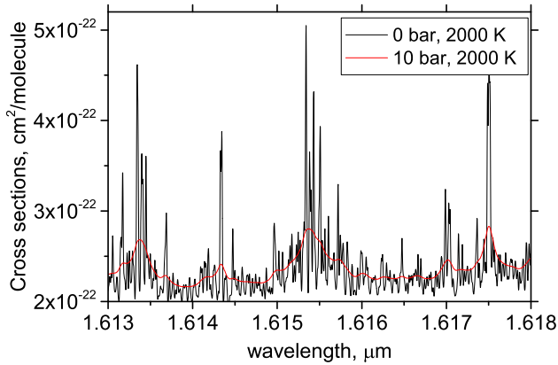
Fig. 7. Comparison of the P = 0 and P = 10 bar line profiles used to generate cross sections at 2000 K in the region of 1.615 μm. The a_0 model with the J -independent line broadening was used. The wavenumber grid \Delta\tilde{\nu} is 0.01 cm −1 .
