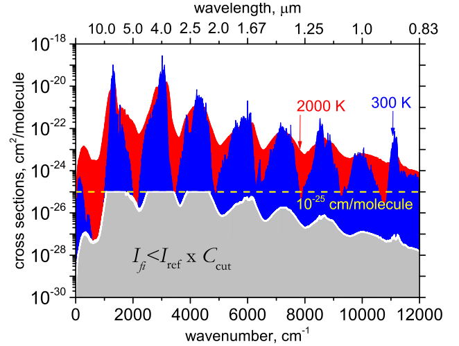
Fig. 3. Intensity partitioning for I_{\text{thr}} = 10^{-25} cm/molecule and C_{\text{scale}} = 10^{-5} . The dashed line indicates the I_{\text{thr}} threshold; the blue ( T = 300 K) and red ( T = 2000 K) areas are the regions of the strong lines; the grey area at the bottom indicates all transitions which were excluded from the line list to form the weak lines of the continuum. Here all cross sections were obtained using the Doppler profile on a grid of 10 cm -1 .
