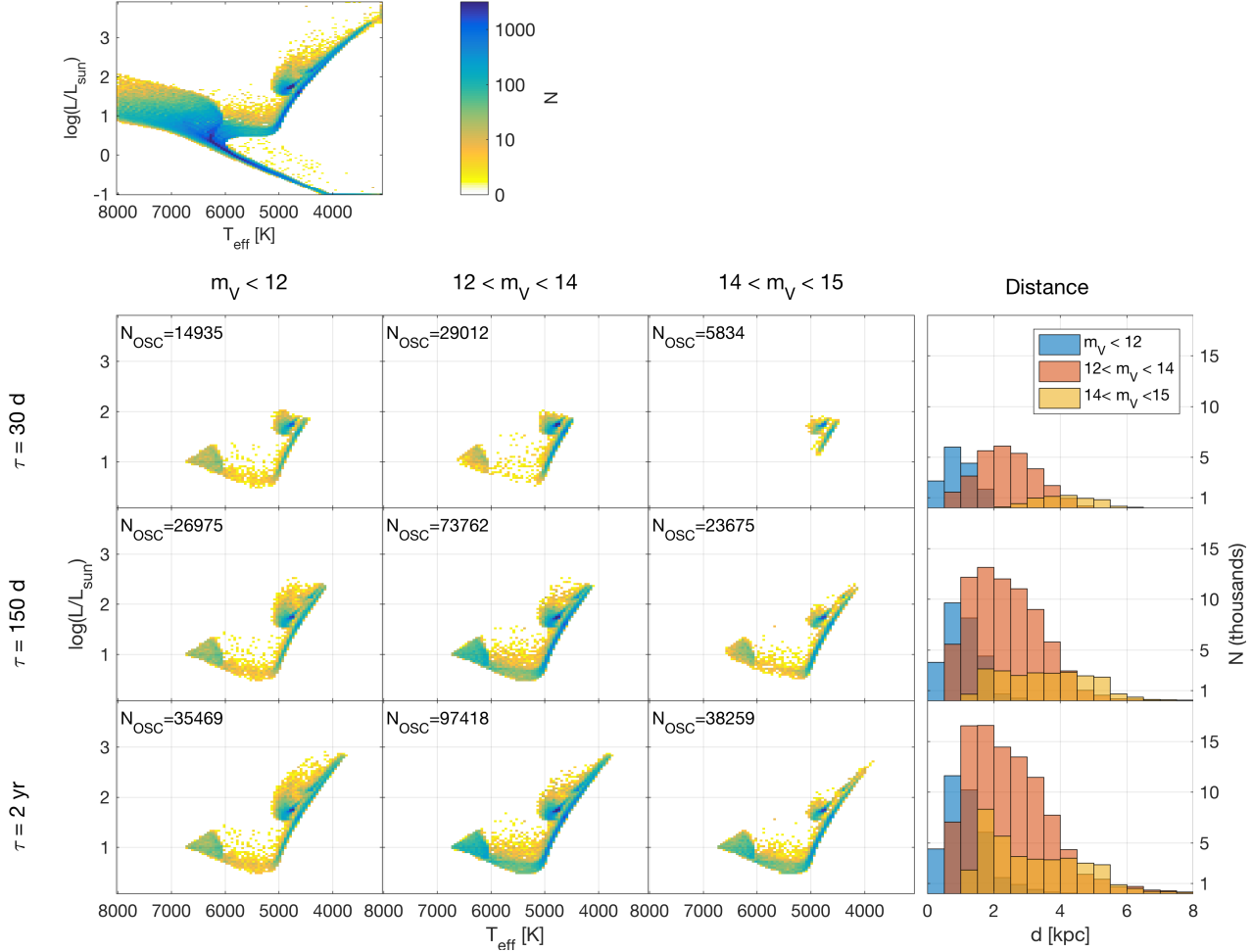
Fig. 3 Upper panel: HR diagram of the synthetic population simulated with TRILEGAL in the PLATO field STEP08. Colour represents the number of stars per T_{\text{eff}}\text{-}\log L bin. Lower panel: In each row we show the HR diagram of stars with detectable oscillations and in different magnitude bins, with N_{\text{OSC}} indicating the approximate number of stars with detectable solar-like oscillations. Our predictions are limited to stars with oscillation frequencies lower than \sim 800 \mu\text{Hz} , hence primarily to stars in the red-giant phase of evolution; see the main text for details. The distance distribution of such stars is presented in the right-most panel. Different rows illustrate the effect of increasing the duration of the observing run, \tau = 30 d, 150 d and 2 yr (first, second, and third row, respectively).
