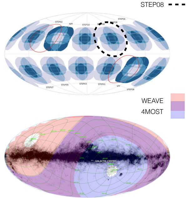
Fig. 2 Upper panel : Projection of the two preliminary long-duration (LD) fields (Southern Plato Field, Northern Plato Field) and ten step-and-stare fields (STEP01 to STEP10), all centred at |b| = 30 , in the Galactic reference frame. The red line is the LD pointing requirement limit. The LD fields are colour-coded on an inverted scale. In the current instrument design various parts of each field are monitored by 24, 18, 12 or 6 cameras (as indicated by different colours). The field selected for this study (STEP08) is encircled by a thick dashed line (Figure taken and adapted from the PLATO Definition Study Report). Lower panel : expected sky coverage of the forthcoming spectroscopic surveys 4MOST and WEAVE superposed on an IRAS map of the sky (Miville-Deschênes & Lagache 2005).
