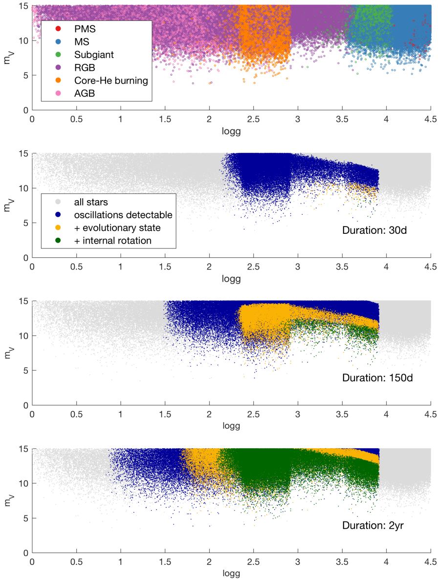
Fig. 4 Stars in the synthetic populations (upper panel of Fig. 3) are presented in a surface gravity versus apparent V -band magnitude plot. The uppermost panel illustrates the location of stars in different evolutionary states (as defined in Bressan et al. 2012), from pre-main-sequence (PMS) to asymptotic-giant-branch (AGB) stars. The other three panels show the expected seismic yields as a function of the duration of the observations, from top to bottom: yields for observations with durations of 30 d, 150 d and 2 yr. Each star in the population is coloured according to the seismic information that can be extracted: gray: no detections, blue: oscillations are detectable (hence \langle \Delta \nu \rangle and \nu_{\max} can be measured), yellow: evolutionary state, based on the detection of the gravity-mode period spacing, can also be inferred, and green: rotationally-split pulsation modes can be measured, hence information on the internal rotational profile can also be inferred. Our predictions are limited to stars with oscillation frequencies lower than \sim 800 \mu\text{Hz} , hence primarily to stars in their red-giant phase of evolution (which are not part of PLATO’s core-target list, see the main text for details).
