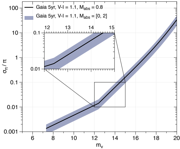
Fig. 8 Gaia’s end-of-mission relative parallax error, evaluated for typical red-giant stars with detectable solar-like oscillations. The solid line illustrates the case of stars with an absolute V -band magnitude representative of red-clump stars. The precision achieved by seismology (few percent) is comparable or better than Gaia’s for stars fainter than m_V = 13 - 14 (i.e. distances \gtrsim 3 kpc, see also Huber et al. 2017). Gaia parallax performance estimate adapted from: https://www.cosmos.esa.int/web/gaia/science-performance (using astrometric error model of de Bruijne et al. 2005 and colour transformation of Jordi et al. 2010).
