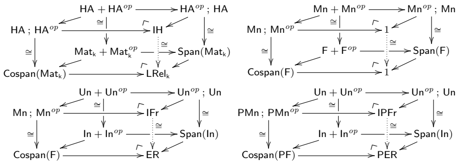
Figure 1. An overview of the various cube constructions considered in this paper. From the top-left corner: the linear case, yielding a characterisation for the PROP LRel_k of k -linear relations (see [5]); the degenerate cartesian case, collapsing to the terminal PROP (Remark 4.11); the (non-degenerate) cartesian case, yielding a characterisation for the PROP ER of equivalence relations (Theorem 4.2); the partial cartesian case, yielding a characterisation for the PROP PER of partial equivalence relations (Theorem 5.4). In the main text we shall write PROPs of spans and cospans in factorised form to emphasise their provenance from distributive laws, e.g. Span(F) as F^{op}; F and Cospan(F) as F; F^{op} .
