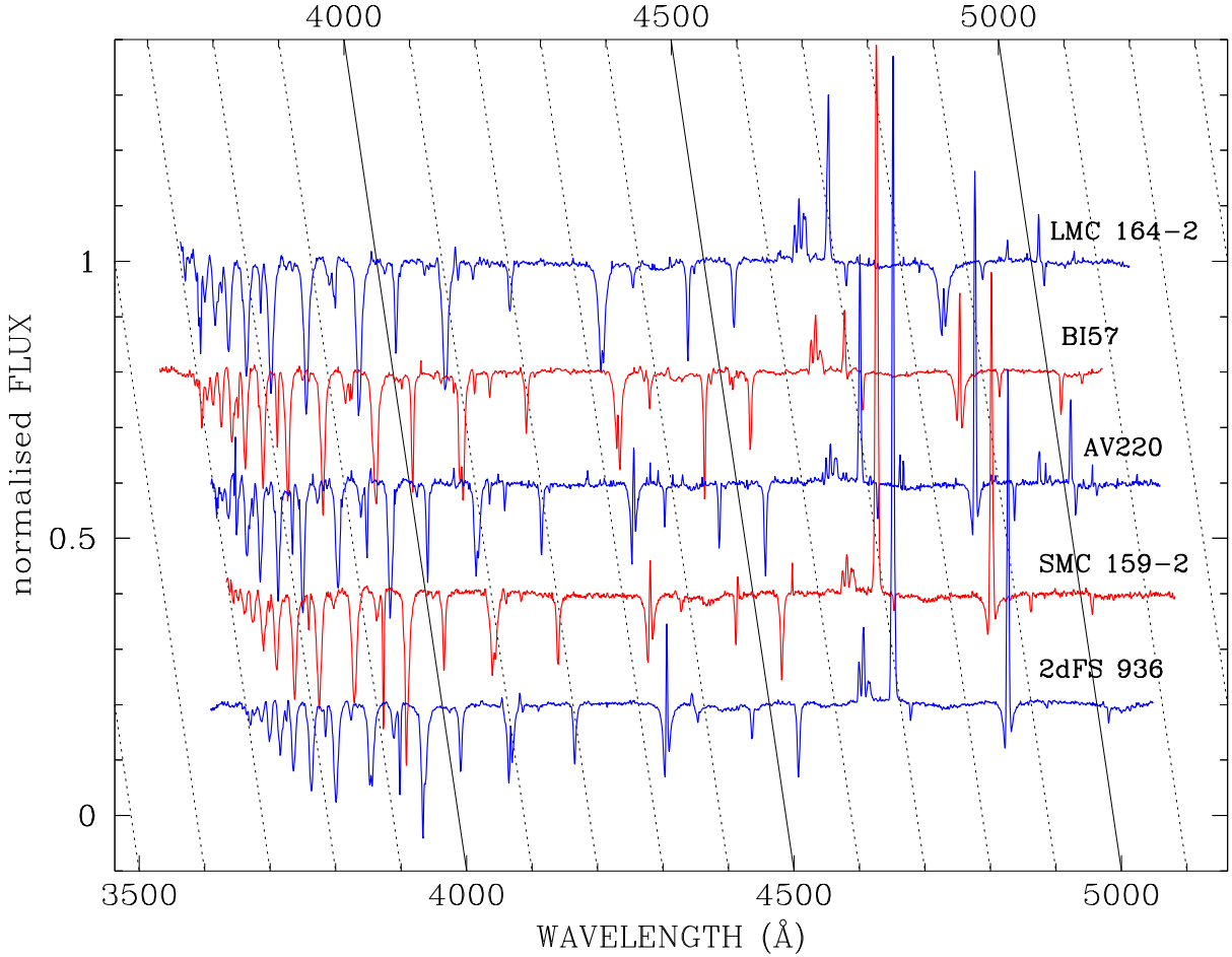
Fig. 3. Normalised FORS2 Stokes I spectra of the five extra-Galactic O-type stars. For display purpose, spectra are offset both in x and y from each other.
