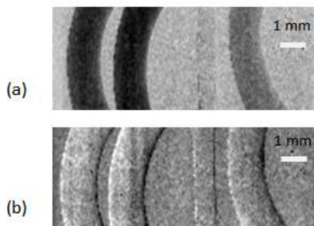
FIG. 6. X-ray absorption (a) and differential phase (b) image of four different rubber cylinders of NBR-70-1, FKM-70, polyurethane, and VMQ-70, respectively from left to right, which were acquired with an EI XPCI system based on the new fabricated metallic glass masks.
