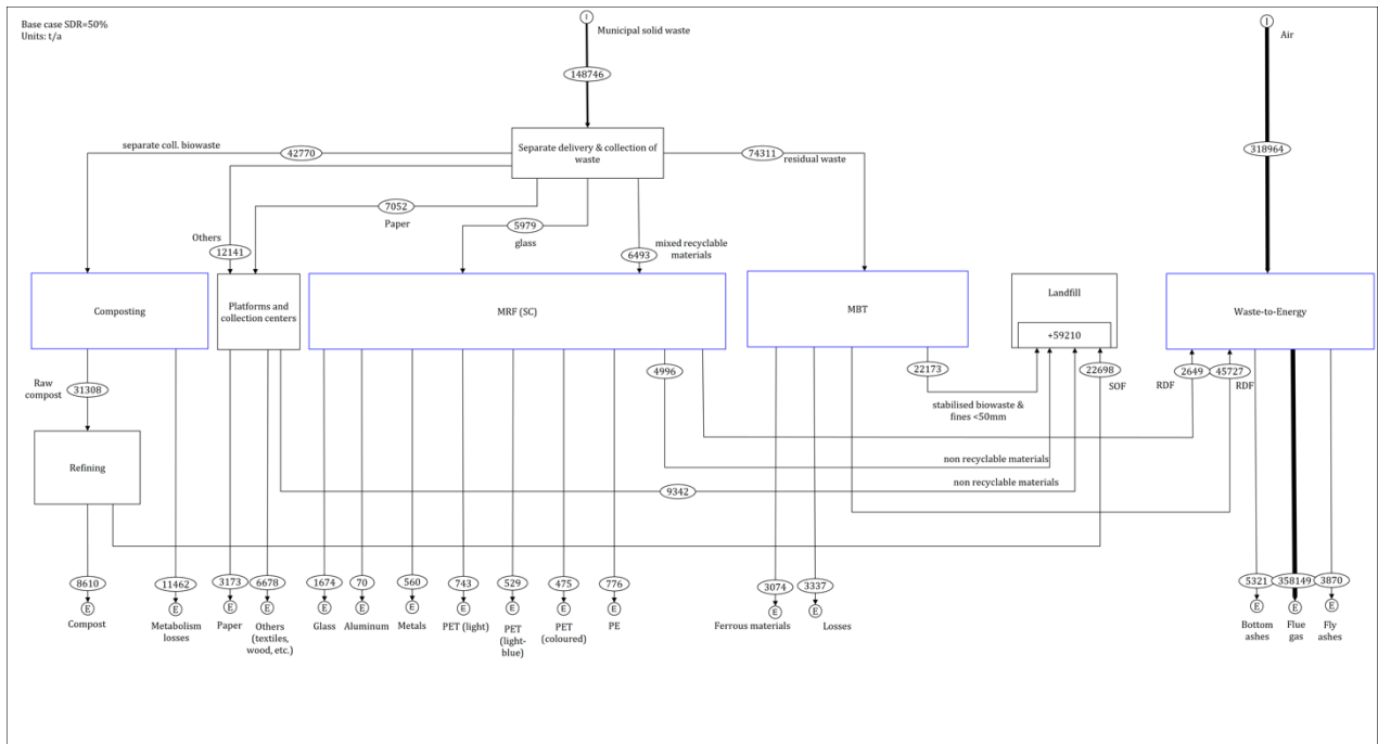
Figure 2: Base case scenario: the graphical representation of the waste management scenario
