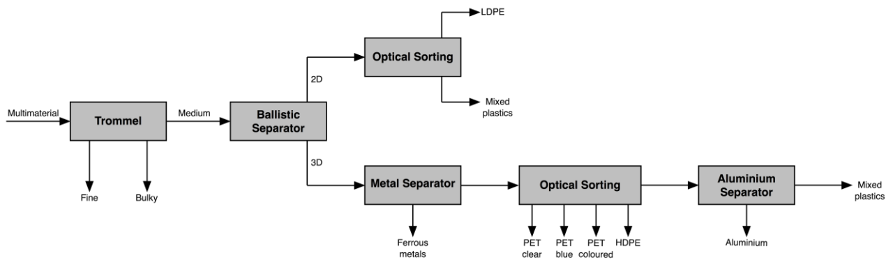
Figure 3: Flow diagram of the MRF sub-system
