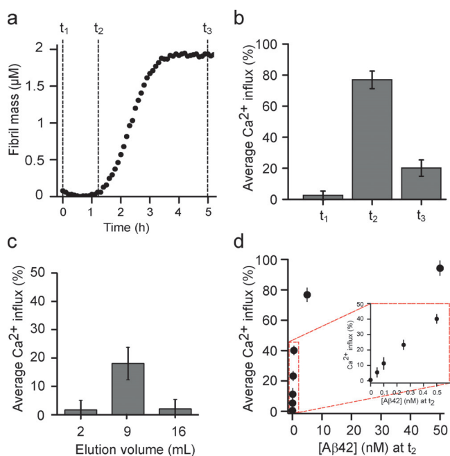
Figure 2. \text{Ca}^{2+} influx caused by aggregates of the \text{A}\beta_{42} peptide. a) Kinetic profile of \text{A}\beta_{42} aggregation under quiescent conditions at a concentration of 2 \mu\text{M} protein. The time points correspond to the start of the aggregation reaction ( t_1 ), the end of the lag-phase ( t_2 ), and the plateau phase ( t_3 ), at each of which an aliquot was taken and diluted to a concentration of 5 \text{ nM} (monomer equivalents). b) \text{Ca}^{2+} influx induced by an aggregation mixture at time points t_1 , t_2 , and t_3 ; a \text{Ca}^{2+} influx of 100% corresponds to the \text{Ca}^{2+} influx caused by ionomycin. c) Size exclusion chromatography of an aliquot taken at t_2 and the degree of \text{Ca}^{2+} influx induced by different elution volumes was then tested. Oligomeric forms of the protein were found to elute at volumes of 7 to 12 mL and monomeric protein at a later elution volume of 14 to 17 mL. d) The dependence of \text{Ca}^{2+} influx on the total concentration of \text{A}\beta_{42} (in monomer equivalents) measured by serial dilution of an aliquot taken at t_2 . The error bars represent variations between different fields of view and the data correspond to averages over measurements of more than 700 vesicles. Inset: expansion of the low concentration region.
