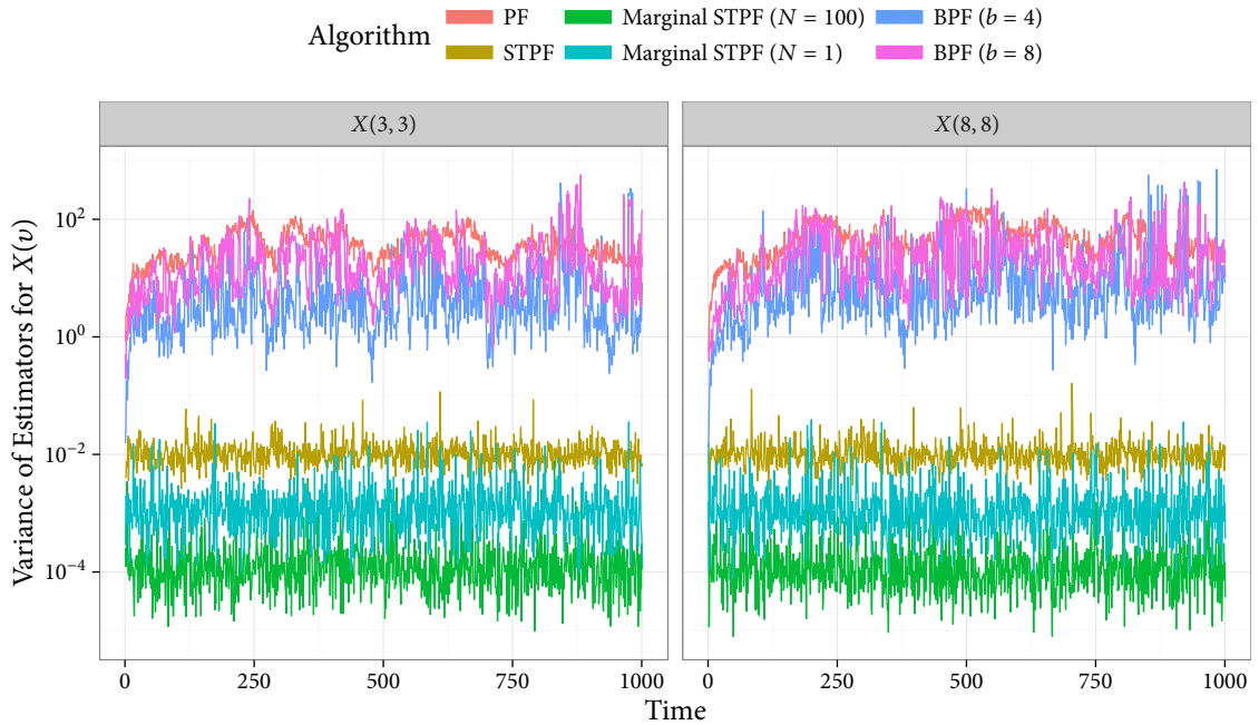
FIGURE 8: Variance plots (on logarithm scale) for estimators of X_n(3, 3) and X_n(8, 8) for Model 2. Variances are estimated from 100 independent runs for each algorithm. STPF uses N = M_d = 100 ; the standard particle filter and BPF use NM_d = 10^4 particles; the two marginal algorithms have used N = M_d = 100 and N = 1, M_d = 1,000 .
