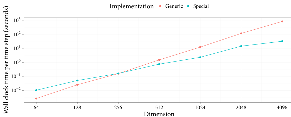
FIGURE 7: Runtime cost of SFTP applied on Model 1 against dimension, for a generic and a ‘special’ implementation of smaller cost. In both cases SFTP used N = 100 , M_d = d .
