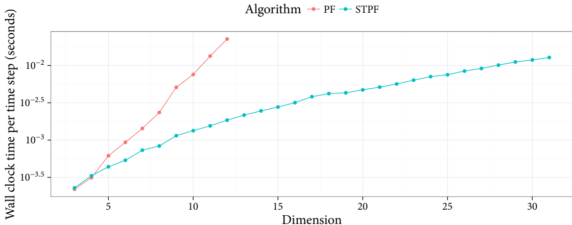
FIGURE 1: Computational cost per time step to achieve a predetermined RMSE versus model dimension, for standard particle filter (PF) and STPF. The two algorithms are applied on Model 1 in Section 4, see Section 4.1 for more details.
