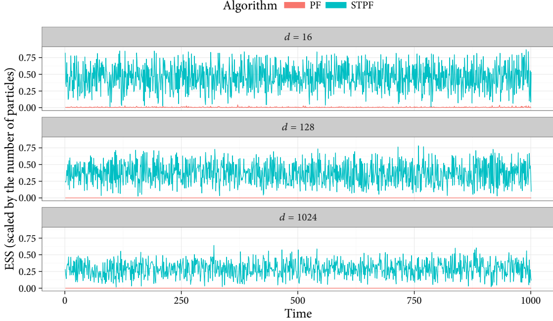
FIGURE 4: Effective Sample Size (ESS) plots for Model 1 from a single algorithmic run.
