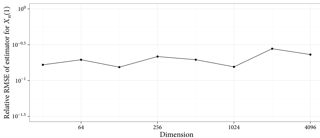
FIGURE 6: RMSE of estimator of \mathbb{E}[X_n(1)|Y_{1:n}] with n = 1,000 , for Model 1 over 100 algorithmic runs (MSE is scaled relatively to the variance of X_n(1)|Y_{1:n} ). We varied d and applied STPF with N = 100 , M_d = d .
