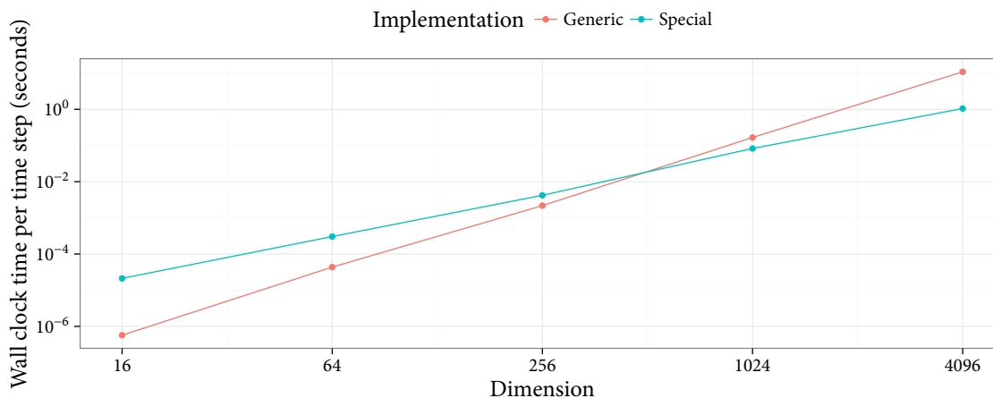
FIGURE 10: Runtime cost of SFTP applied on Model 2 against dimension, for a generic and a ‘special’ implementation of smaller cost. In both cases, SFTP used N = 100 , M_d = d/8 .
