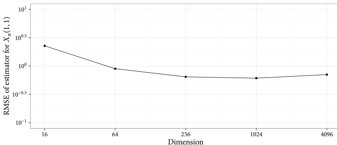
FIGURE 9: RMSE of estimators of \mathbb{E}[X_n(1, 1)|Y_{1:n}] with n = 1,000 , for Model 2, over 100 algorithmic runs. We applied STPF with N = 100 , M_d = d/8 , and varying dimension d .
