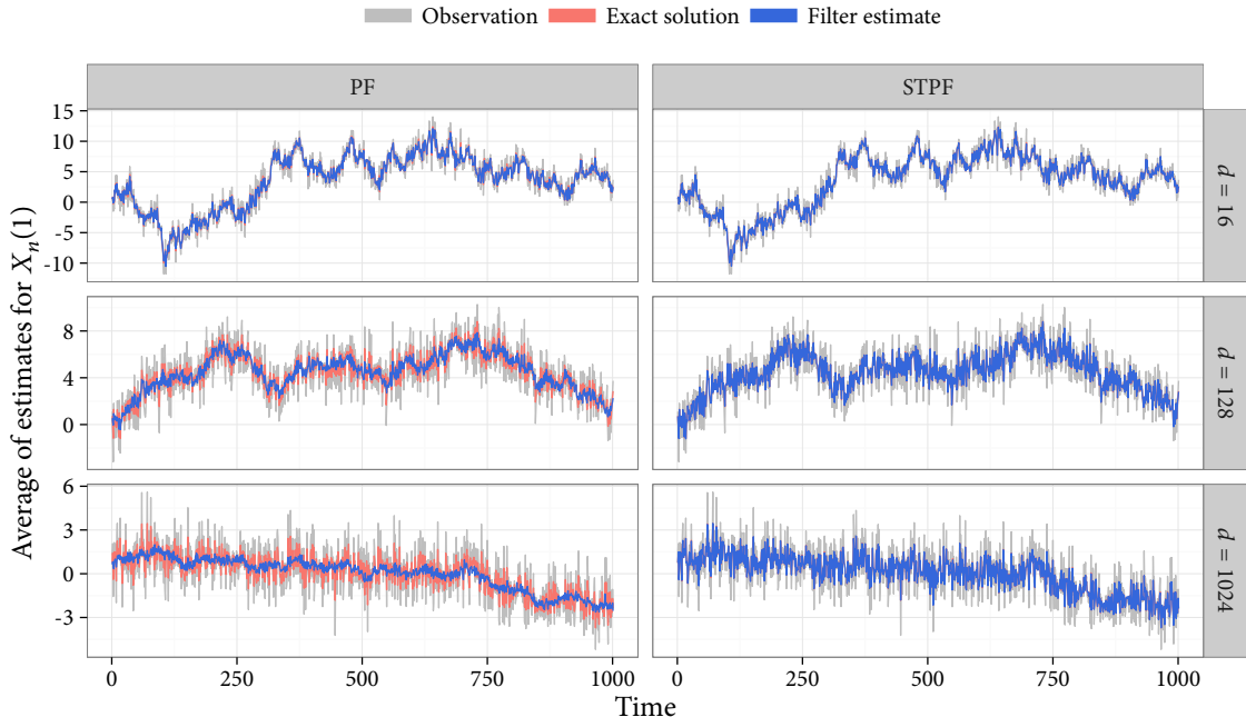
FIGURE 3: Average of estimators of \mathbb{E}[X_n(1)|Y_{1:n}] for Model 1 across 100 algorithmic runs.
