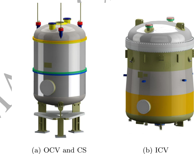
Figure 1: CAD models of the cryostat vessels and support. The OCV connects to three support legs mounted on baseplates and the ICV will be placed inside the OCV in vacuum. The full cryostat assembly stands 4.1 m tall.
