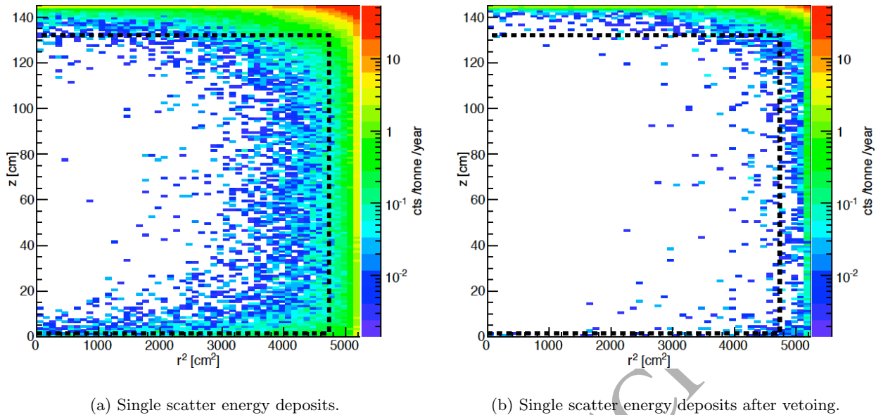
Figure 2: Expected background from the cryostat in LZ, showing the spatial distribution in r^2 and z within the active volume, and the fiducial volume (black dashed) that contains 5.6 tonnes of LXe. The colour scales are in counts/tonne/year. The effect of vetoing is highlighted through the reduction of events that satisfy single scatter selection in the energy range of interest for a WIMP search (left) by a factor \sim 10 when vetoes are implemented (right).
