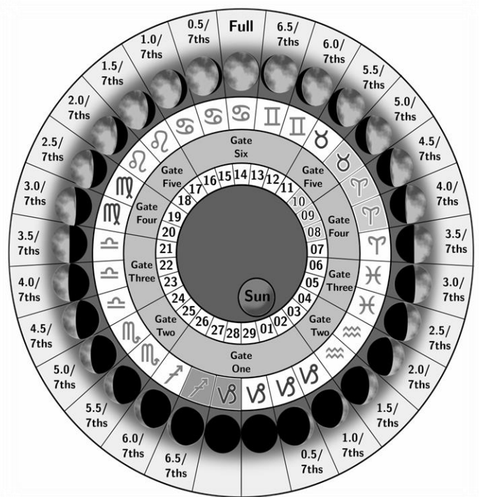
Figure 1: Basic diagram to illustrate moonrise data in 4Q209 column iii: the days of the month are in the inner circle. The text describes the waxing movements of the moon on Nights 8 to 10, entering Gate 5 (days shaded). The Sun travels in Gate 1 at the same time. The moon enters Gate 5 after sunset on Night 9 and rises in Gate 5 on Day 10
