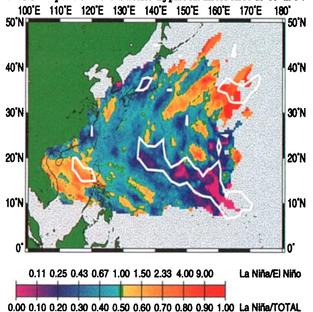
ENSO Impact on NW Pacific Typhoon Incidence 1965-1997
