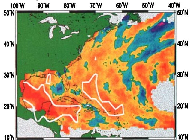
ENSO Impact on Atlantic Hurricane Incidence 1900-1997
