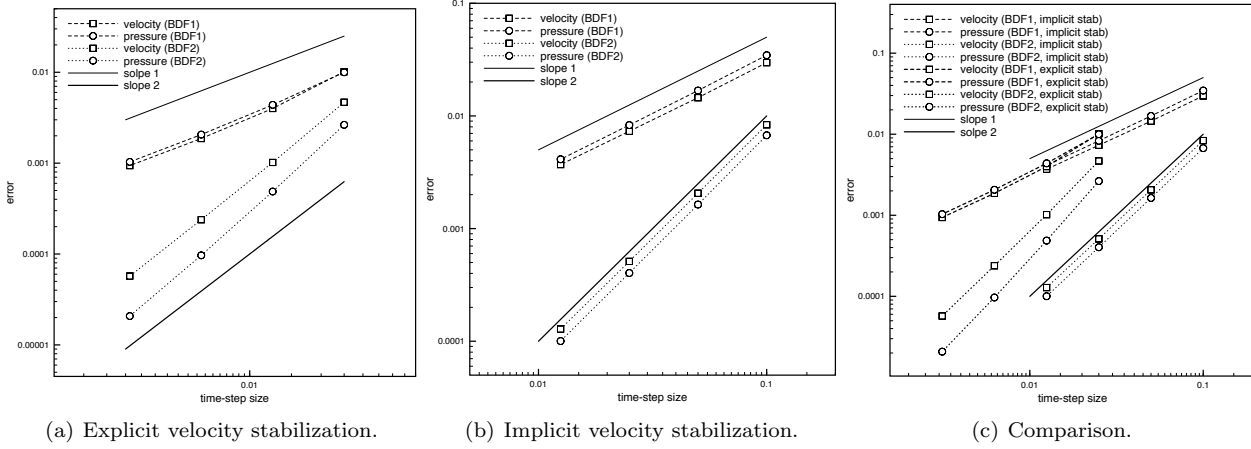
FIGURE 1. Convergence plot for the fractional-step method applied to the problem defined by the exact solution (57). Dotted (resp., dashed) lines correspond to the fractional-step method using BDF2 (resp., BDF1). Solid lines mark first- and second-order slopes. Square markers indicate L^2 -norm errors on the velocity and circle markers indicate L^2 -norm errors on the pressure. In (c) all the curves are collected in one graph for comparison.
