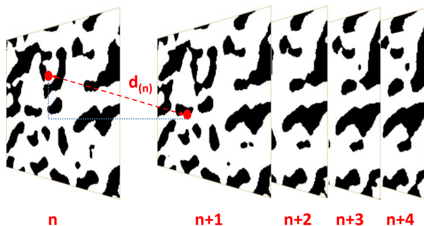
Figure 8: Illustration of the pore centroid method calculation approach which measures the distance d_{(n)} of the centres of mass between two 2D image slices
