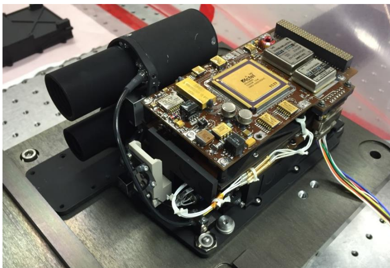
Figure 1: UVIS Flight Model instrument under test
