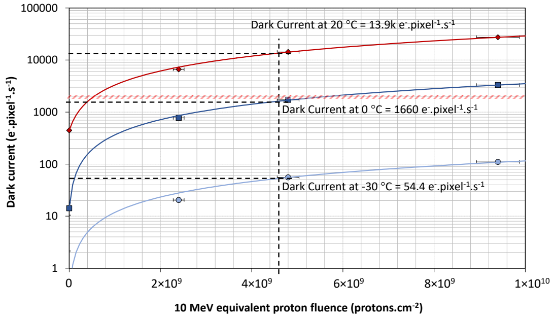
Figure 7: Dark current at 20°C, 0 °C and -30 °C as a function of proton fluence showing the desired dark current limit at 0 °C for the CCD operational lifetime at a factor 1.2 times that of the predicted end of life fluence
