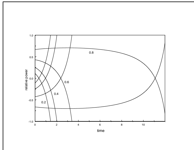
Figure 7 Variation of p_1(t) and p_2(t) for N_2 = 1000 and N_1 = 800, 600, 400 \text{ \& } 200 during an asymmetric conflict with a ‘search’ probability D_I = 0.0003 . Each pair of lines cross in this example, indicating that rebel victory occurs in all cases
