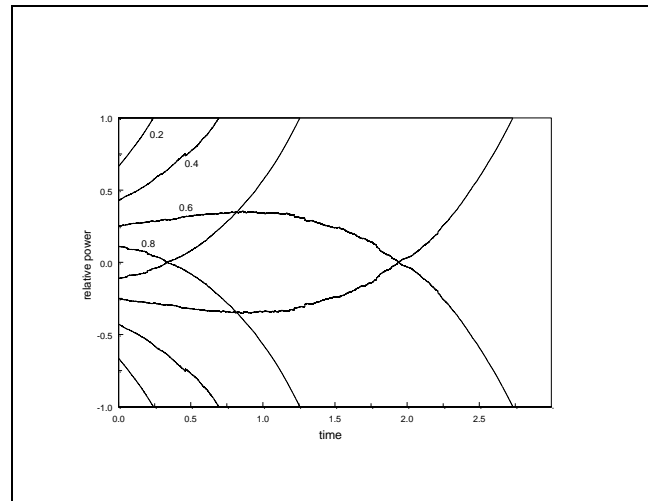
Figure 12 Variation of p_1(t) and p_2(t) for N_2 = 1000 and N_1 = 800, 600, 400 \text{ \& } 200 during a direct-fire conflict with a stochastic element applied to the rebel groups only ( N_I ). Rebel victory ensues for the two largest rebel groups
