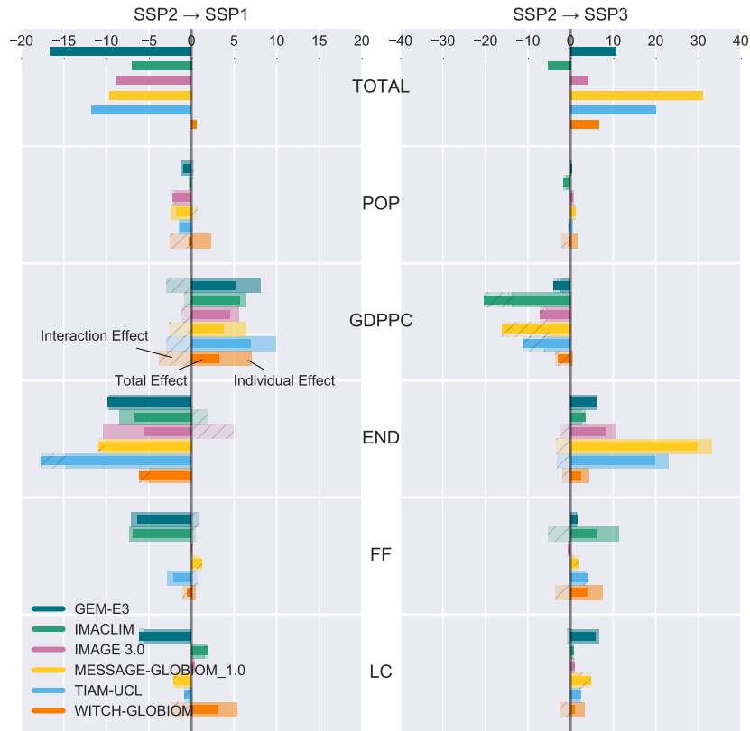
% Change in Cumulative CO 2 Fossil Fuels Emissions 2010-2050 wrt SSP2 under CPRICE
