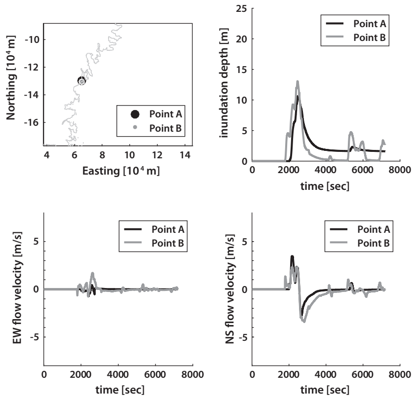
Fig. 5. Simulated wave traces in two different locations in Kesenuma Bay area.
