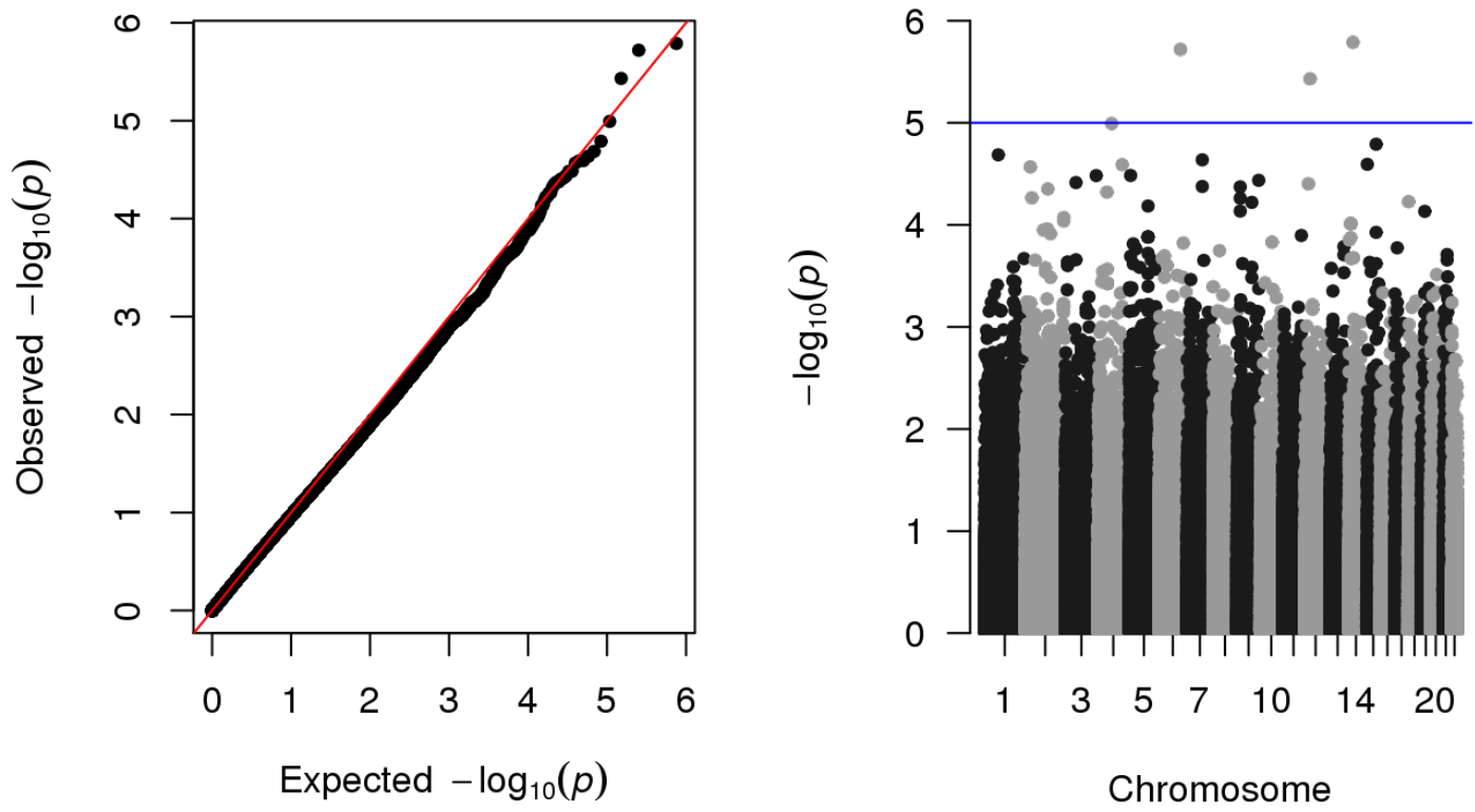
Supplementary Figure 4: Quantile-Quantile and Manhattan plots of GWAS results of the FHS \Delta BMI phenotype in lung cancer case
