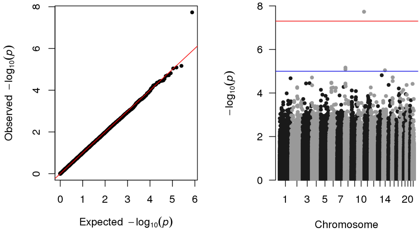
Supplementary Figure 3: Quantile-Quantile and Manhattan plots of GWAS results of the FHS \Delta BMI phenotype in GI cancer cases
