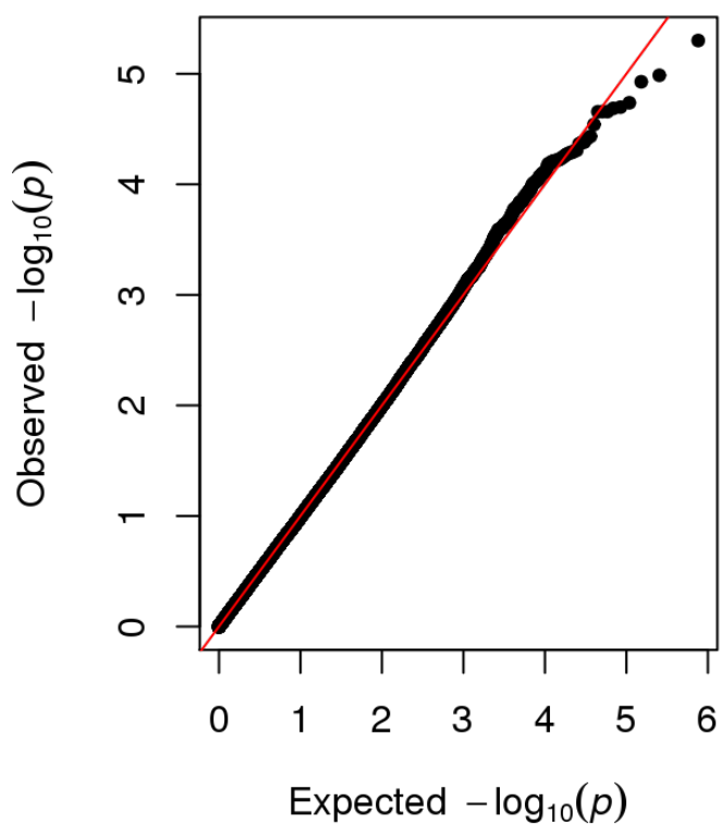
Supplementary Figure 1: Quantile-Quantile and Manhattan plots of GWAS results of the FHS \Delta BMI phenotype in any cancer cases
