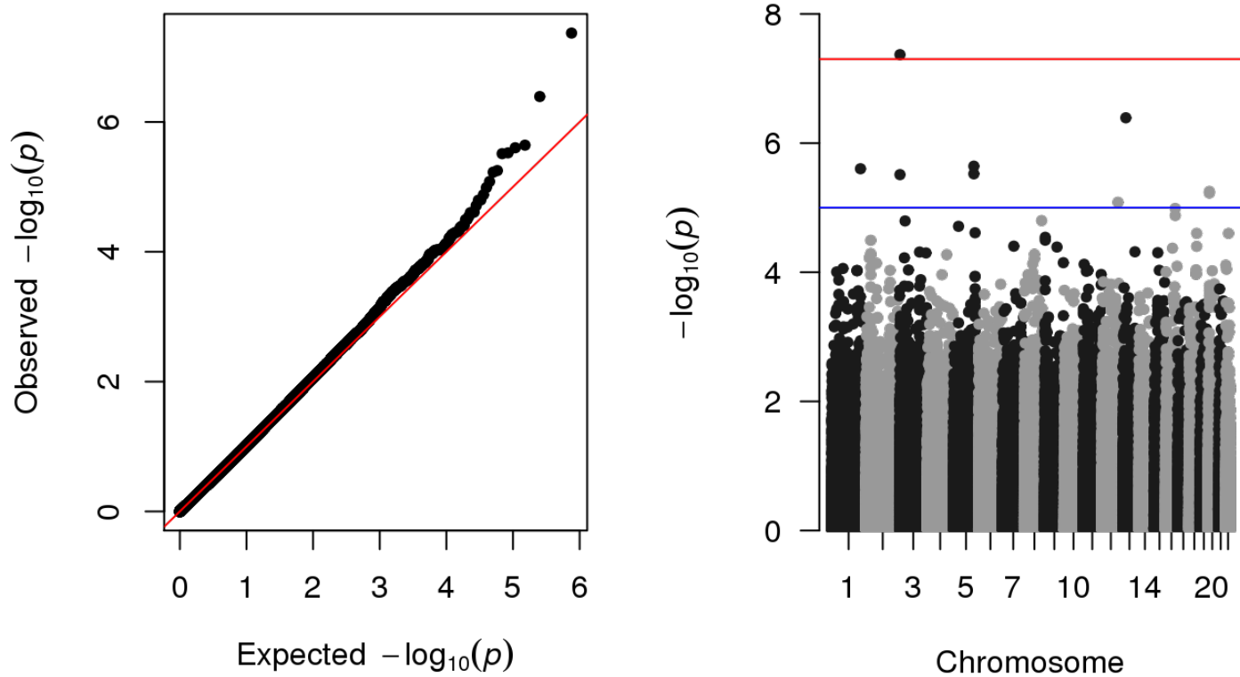
Supplementary Figure 2: Quantile-Quantile and Manhattan plots of GWAS results of the FHS \Delta BMI phenotype in COPD cases
