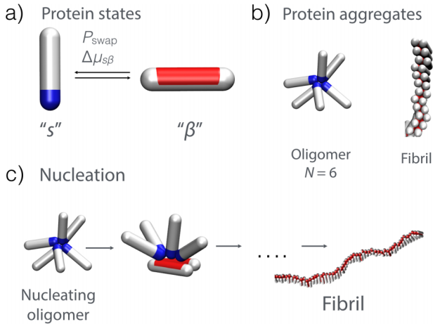
FIG. 2. The Monte Carlo model. (a) The protein can switch between two states: the soluble state, "s," that is lower in energy, interacts weakly with its own kind, and forms disordered oligomers and the \beta -sheet prone state, "β," which is higher in energy, but interacts stronger with its own type than the soluble state, and forms fibrils. Attractive patches are coloured in blue and red for the "s" and "β" state, respectively. (b) Aggregates of the two possible states: disordered oligomer (left panel) and fibril (right panel). (c) At low protein concentrations nucleation proceeds via oligomers. Illustration of an oligomer of size N=6 , where the nucleation takes place when two proteins simultaneously convert into the \beta -prone state, which triggers the nucleus growth into a long fibril.
