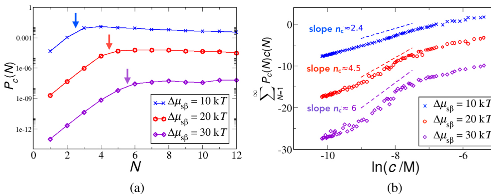
FIG. 5. (a) The calculated probability of “s” → “β” conversion per MC step of a single protein within an oligomer of the size N , for three different \beta -propensities, from top to bottom: \Delta\mu_{s\beta} = 10kT , \Delta\mu_{s\beta} = 20kT , and \Delta\mu_{s\beta} = 30kT . The arrows mark the respective saturation of the conversion probability. (b) The calculated rate, from Eq. (13), for three different \beta -propensities.
