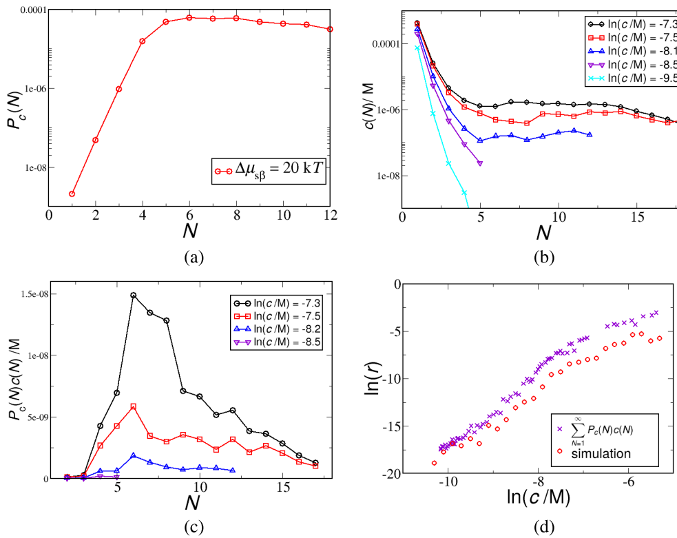
FIG. 4. (a) The calculated probability of “s” → “β” conversion of a single protein within an oligomer of the size N , for the protein with a low \beta -propensity, \Delta\mu_{s\beta} = 20kT , per MC step. (b) Steady-state concentration of “s”-state oligomers of size N for five different protein concentrations. (c) Product of a conversion probability within an oligomer of a size N per MC step, from (a), with the concentration of the oligomers of size N , from (b). (d) The calculated rate: Sum of the concentrations of all oligomers multiplied by the corresponding protein conversion rates within an oligomer, across the concentration range, as in Eq. (13). The nucleation rate measured in simulations for the same set of parameters is shown for comparison (red circles), taken from Fig. 3(a).
