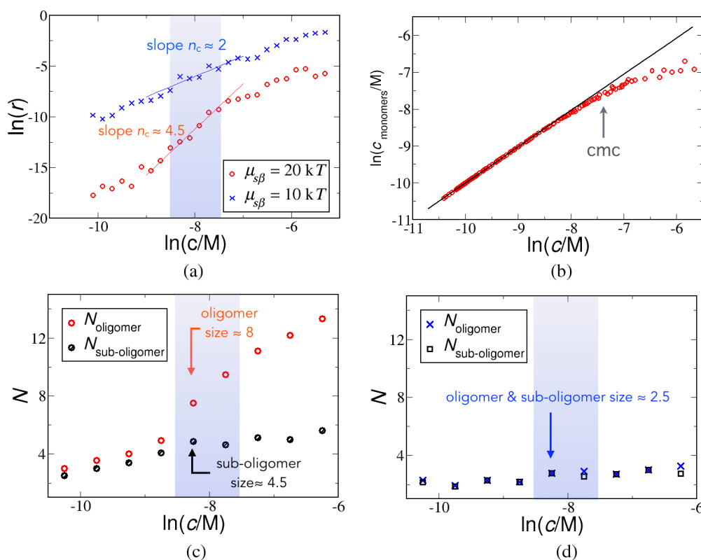
FIG. 3. Kinetics of nucleation via oligomers from Monte Carlo simulations. (a) The rate of nucleation versus protein concentration measured in simulations, for proteins with low propensity for \beta -sheet ( \Delta\mu_{s\beta} = 20\text{kT} , red circles) and high \beta -sheet propensity ( \Delta\mu_{s\beta} = 10\text{kT} , blue crosses). (b) The concentration of free monomers in solution versus the total protein concentration. The solid line has the slope of 1, and the dashed line indicates the critical micelle concentrations. (c) The average size of the overall nucleating oligomer (red circles) for the low \beta -propensity protein ( \Delta\mu_{s\beta} = 20\text{kT} from (a)), and the average size of the sub-oligomer participating in the conversion step (black circles). (d) The average sizes of the overall nucleating oligomer (blue crosses) and the sub-oligomer participating in the conversion step (black squares) for the high \beta -propensity protein ( \Delta\mu_{s\beta} = 10\text{kT} from (a)).
