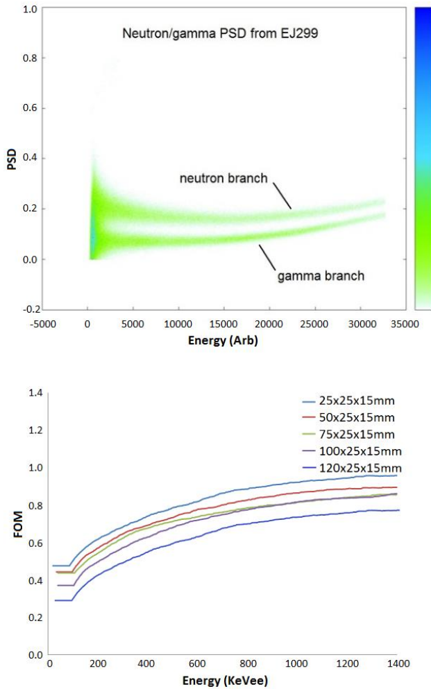
Fig. 5. (top) 2D plot, for a 25x25x15mm piece of EJ-299-34, of PSD against energy for an Am/Be mixed n/ \gamma flux, (bottom) PSD FOM as a function of photon energy for a range of EJ-299-34 scintillator geometries
