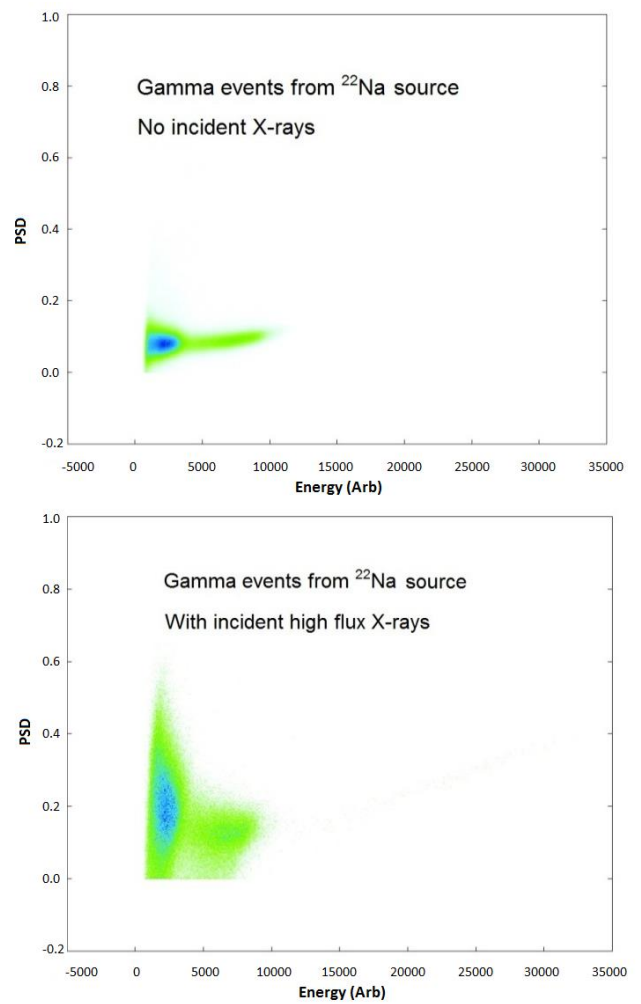
Figure 6: 2D plots of PSD vs energy for gamma events from ^{22}\text{Na} . (top) without X-ray irradiation, (bottom) with simultaneous high flux X-ray irradiation.
