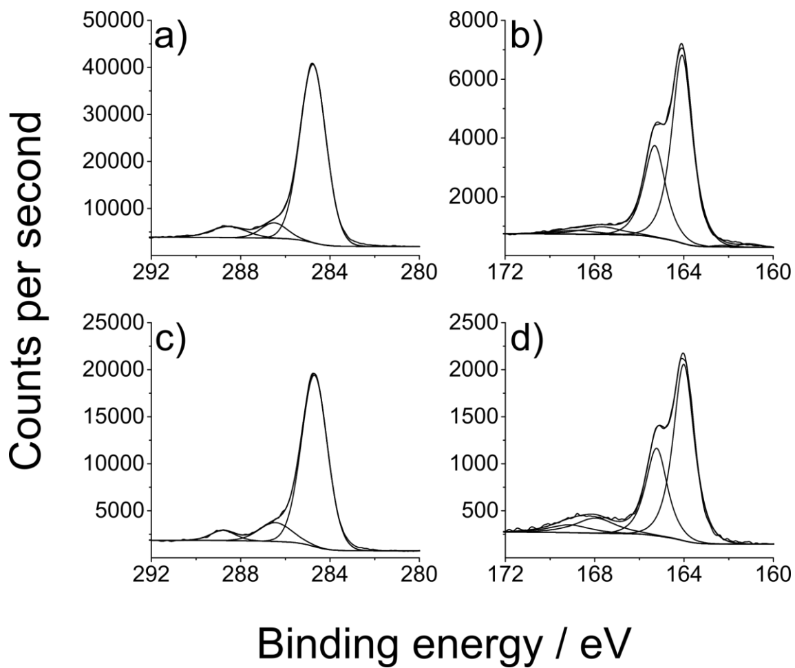
Figure 3. High resolution XPS scans of C1s and S2p of 10 wt. % and 50 wt. % DIB content sulfur polymers after carbonisation: a) 10 wt % C1s, b) 10 wt. % S2p, c) 50 wt. % C1s and d) 50 wt. % S2p.
