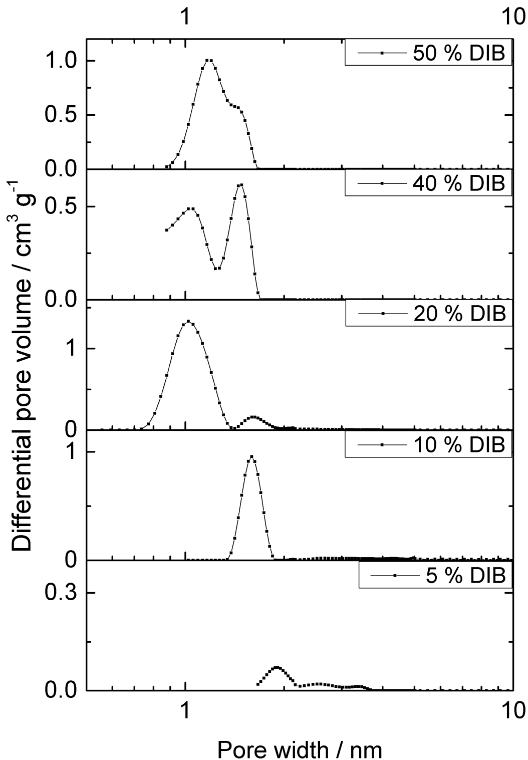
Figure 5. (b) NL-DFT pore size distribution, calculated from the nitrogen isotherms, for a series of carbonised S-DIB copolymers.
