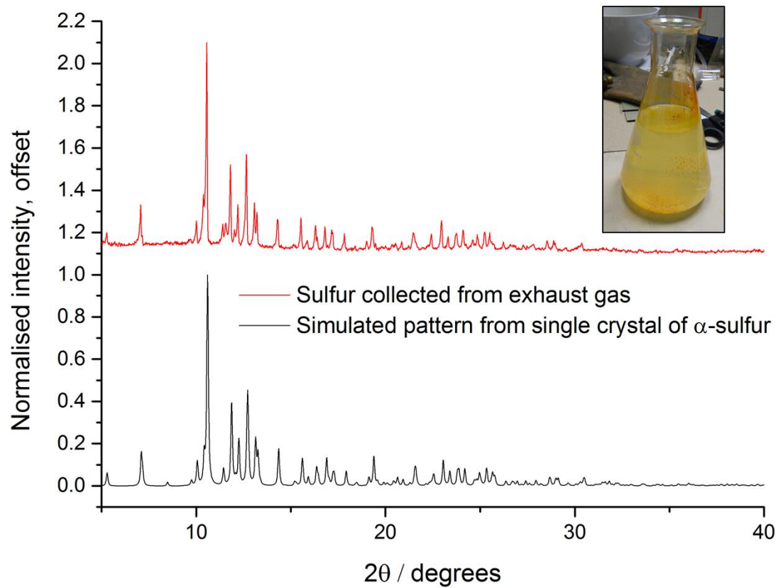
Figure S2. Powder XRD of the yellow precipitated powder collected from water through which the exhaust gas was bubbled (inset). As can be seen, the experimental pattern matches the common \alpha form of elemental sulfur.
