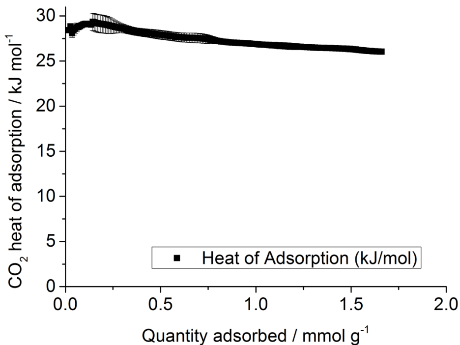
Figure S5. Isosteric heat ( Q_{st} / kJ mol -1 ) of adsorption for CO 2 as a function of the amount adsorbed (mmol g -1 ) for the temperature range 263–298 K, determined using the standard calculation routines in the Data-master offline data reduction software (Micromeritics), for 10 wt. % DIB carbonised S-DIB.
