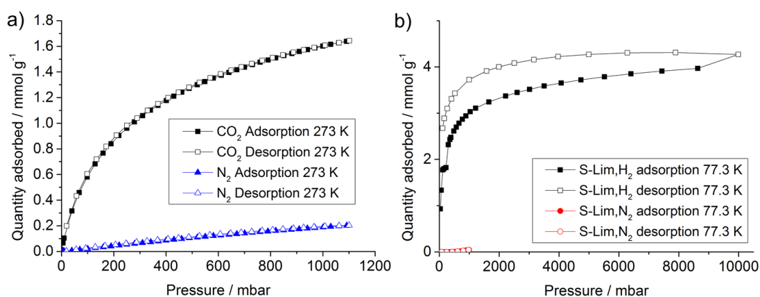
Figure 6. a) Adsorption isotherms (solid symbols) and desorption isotherms (open symbols) for carbon dioxide and nitrogen on carbonised S-Lim (50 wt% limonene), up to 1 bar pressure and at 273 K. b) Adsorption isotherms (solid symbols) and desorption isotherms (open symbols) for hydrogen and nitrogen on carbonised S-Lim (50 wt% limonene), up to 10 bar pressure and at 77.3 K.
