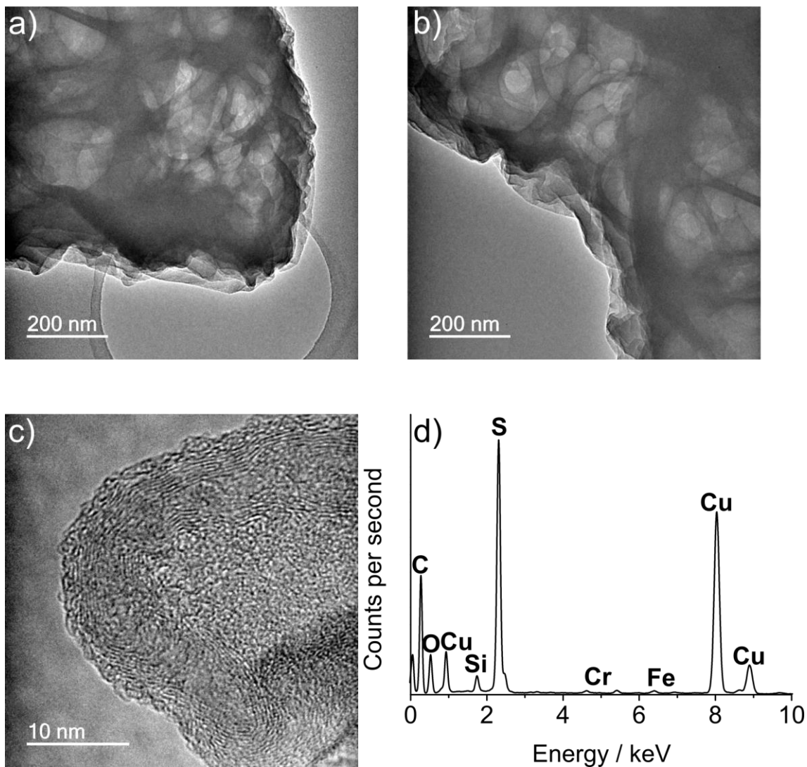
Figure 2. TEM images of a carbonised sample of S-DIB (40 wt% DIB). Images a) and b) show the internal voids in the structure, from removal of sulfur during carbonisation. HRTEM, c), reveals some degree of local order and crystallinity in the carbonised material. EDS analysis, d), indicates the presence of carbon and sulfur. It should be noted that copper emanates from the copper sample grid and chromium and iron emanate from the steel sample holder.
