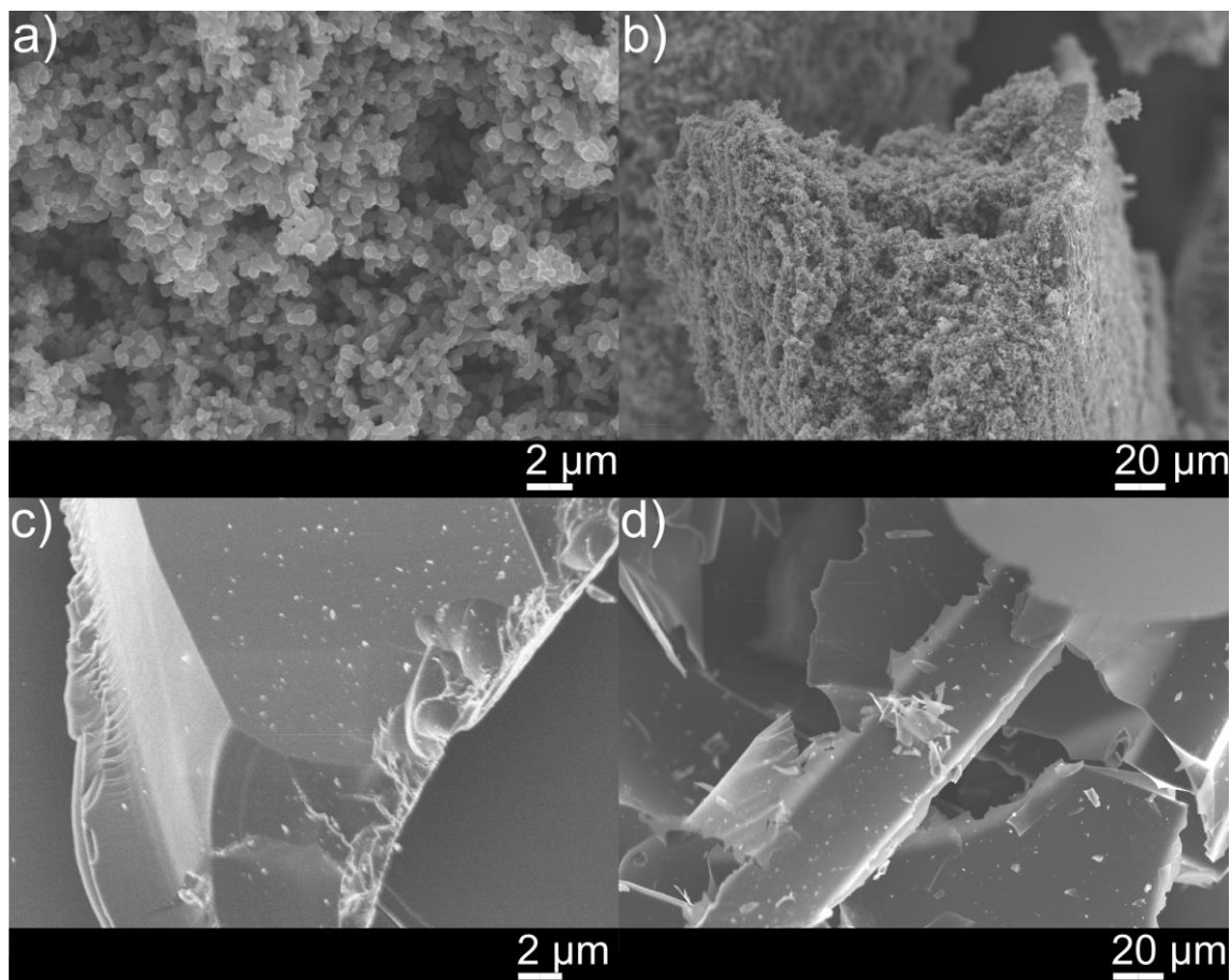
Figure 1. SEM images of: a) and b) high sulfur (90 wt. % S) polymer showing the porous microstructure of the monolith and c) and d) as the smooth, low sulfur (50 wt. % S) polymer sample, showing the smooth architecture.
