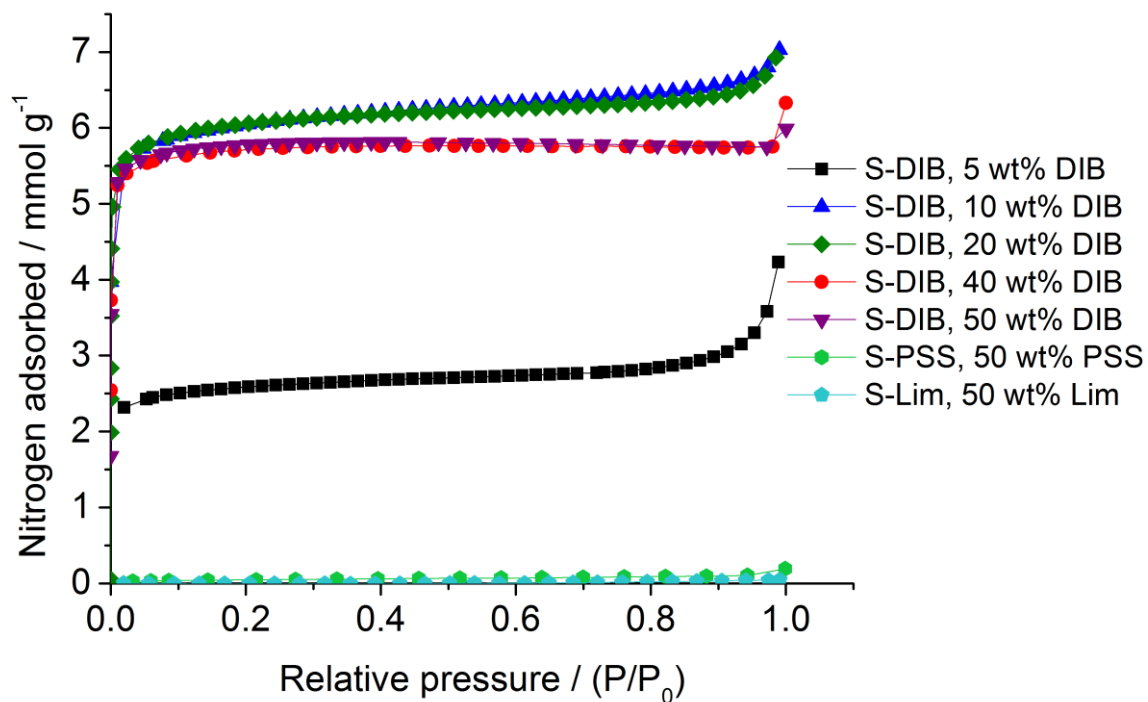
Figure 4. Nitrogen adsorption isotherms (at 77.3 k, 1 bar) of carbonised samples of S-DIB polymers, as well as S-limonene copolymer (S-Lim) and a sulfur-poly(4-styrenesulfonate) mixture (S-PSS).
