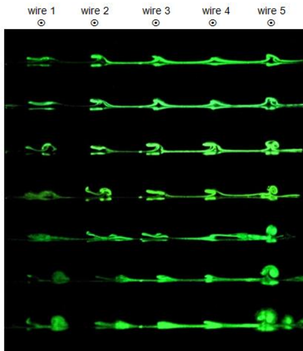
Fig. 3 Evolution of the vortices induced by a series of 5 perturbation wires of diameter 0.7 mm for Re = 2500, 3500, 4250, 5500, 6250, 6500, \text{ and } 7000 (top to bottom) at the first peak of corrugation with S = 0.250
