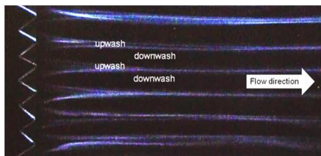
Fig. 5 Linear smoke streaklines from the top view of the entrance flat plate before the corrugation at Re = 3500 . Air is flowing from left to right
