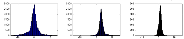
Fig 3. SAS value histograms – 2 nd Order “good” shim. Uncorrected, WASSR and GRE respectively
