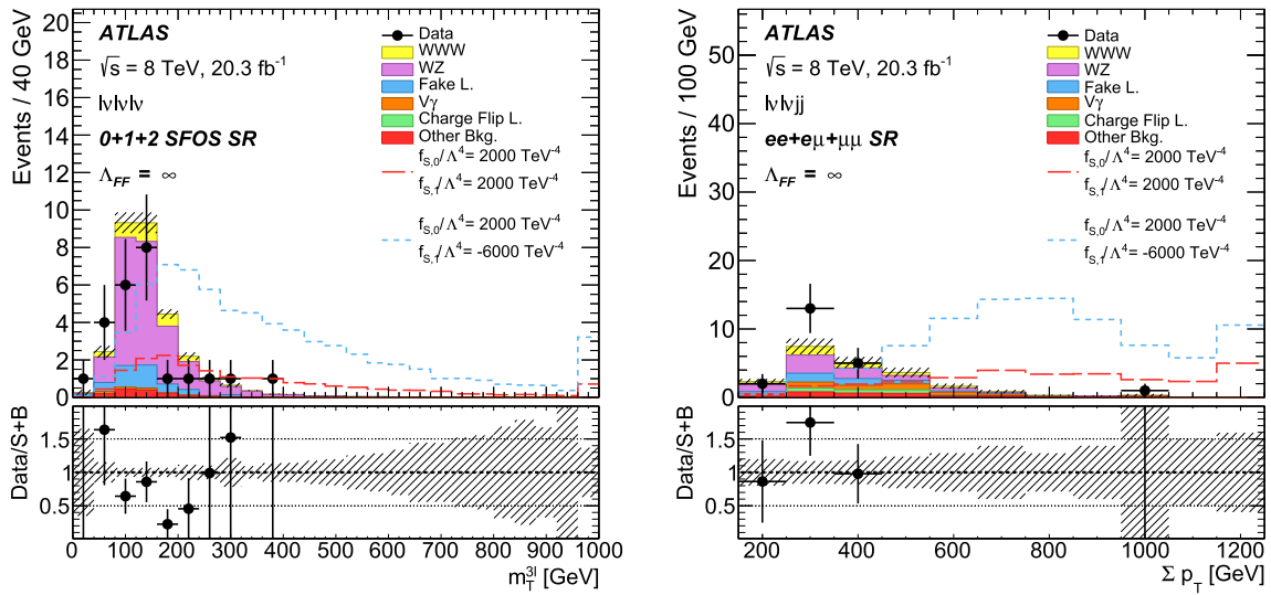
Fig. 3 The distribution of m_T^{3\ell} for the l\nu l\nu l\nu channel (left) and the distribution of \Sigma_{PT} for the l\nu l\nu jj channel (right) as observed in the data (dots with error bars indicating the statistical uncertainties) and as expected from SM signal and background processes. The ratios between the observed numbers of events in data and the expected SM signal plus background contributions are shown in the lower panels. The hashed bands results from the systematic uncertainties on the
