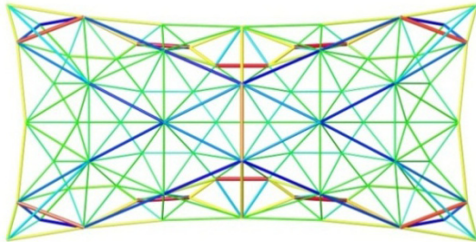
Figure 8. Optimal Force Distribution
