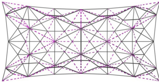
Figure 12. Most Efficient Actuators Pattern
