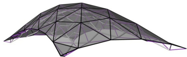
Figure 3. Catenary Dome, Perspective
