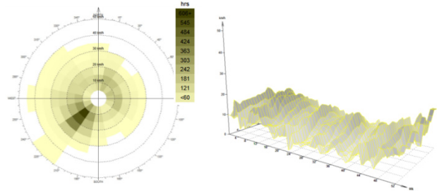
Figure 6. Wind Velocities and Frequency
