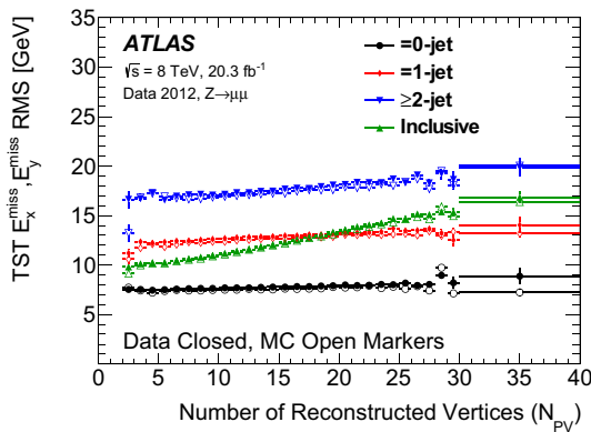
Fig. 8 The resolution of the combined distribution of E_T^{\text{miss}} and E_Y^{\text{miss}} for the TST E_T^{\text{miss}} as a function of N_{PV} for the 0-jet, 1-jet, \geq 2 -jet, and inclusive Z \rightarrow \mu\mu samples. The data (closed markers) and MC simulation (open markers) are overlaid. The jet counting uses the same JVF criterion as the TST E_T^{\text{miss}} reconstruction algorithm
