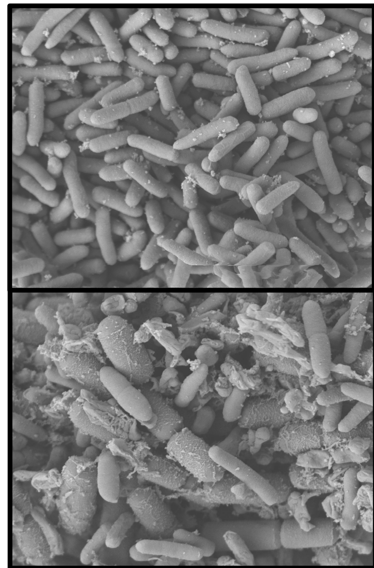
Figure 1: Scanning Electron Microscopy (SEM) images at x10,000 magnification, at early and late stage stationary phase.
