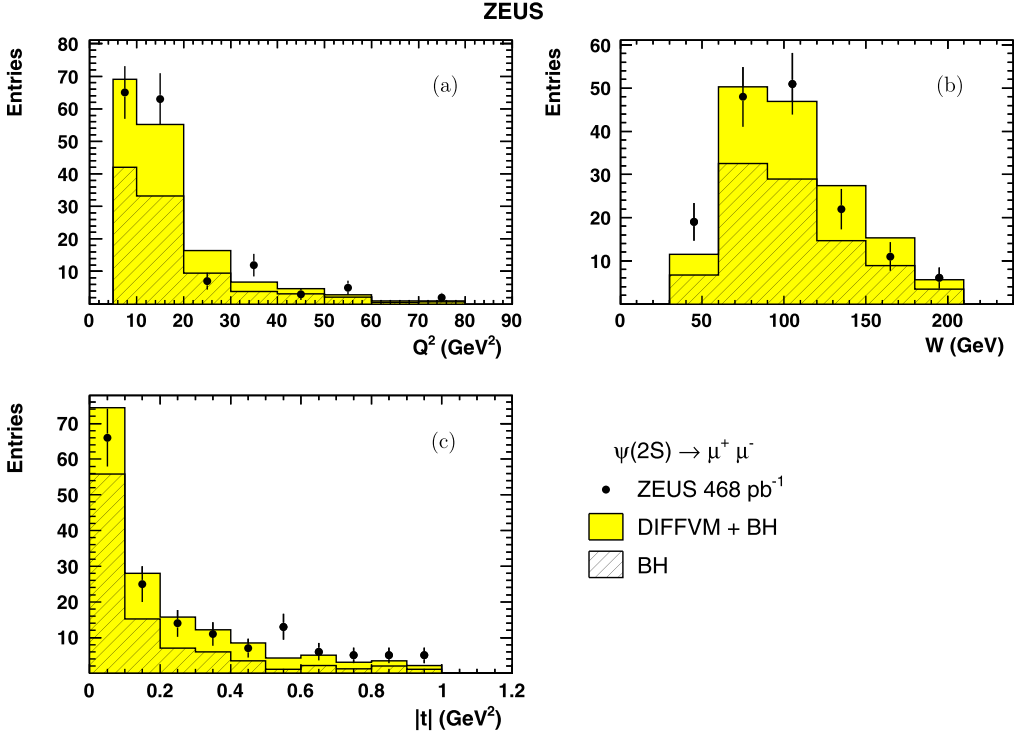
Fig. 5. Comparison of the measured (points with statistical uncertainties) and the reweighted simulated distributions (shaded histograms) for the \psi(2S) \rightarrow \mu^+\mu^- events as a function of (a) Q^2 , (b) W and (c) |t| . The mass range 3.59 < M_{\mu\mu} < 3.79 GeV was selected. The hatched histogram shows the contribution of the simulated Bethe–Heitler background.
