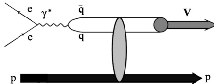
Fig. 1. Schematic representation of the exclusive electroproduction of q\bar{q} vector mesons. The electron emits a virtual photon, which fluctuates into a q\bar{q} pair. The q\bar{q} pair interacts with the target proton and produces the q\bar{q} vector meson V .
