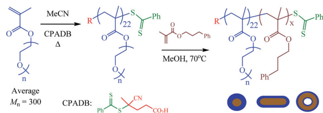
Scheme 1 General approach for the preparation of poly[oligo-(ethylene glycol) methyl ether methacrylate- block -3-phenylpropyl methacrylate]-based nanoparticles by methanolic RAFT dispersion polymerization with polymerization-induced self-assembly.
