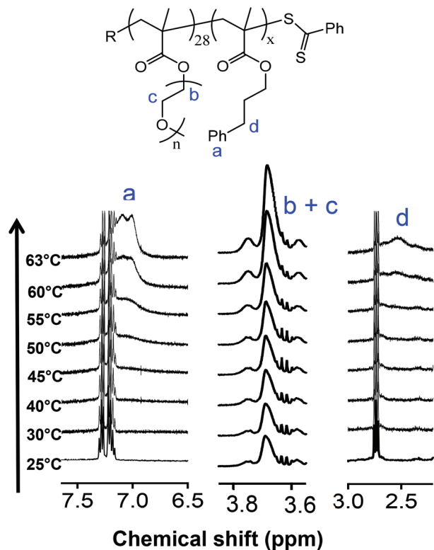
Fig. 2 General structure of the p(OEGMA 28 - block -PPMA x ) copolymers (top) and a series of 1 H NMR spectra covering the temperature range 25–63 °C (bottom) highlighting the increase in solvation of key functionality associated with both the pOEGMA coronal and pPPMA core blocks with increasing temperature. Spectra were recorded in d 4 -methanol.
