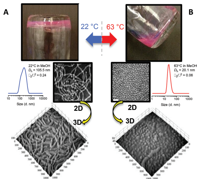
Fig. 1 (A) Digital picture of the macroscopic presentation of the p(OEGMA 28 - block -PPMA 69 ) copolymer worm nanoparticles at 22 °C with representative 2D and 3D TEM images below and the DLS-measured nanoparticle size distribution, and (B) the same sample after heating to 63 °C highlighting the change in macroscopic presentation with the 2D/3D TEM images of the new, predominantly, spherical nanoparticles and the concomitant change in the DLS nanoparticle size distribution.
